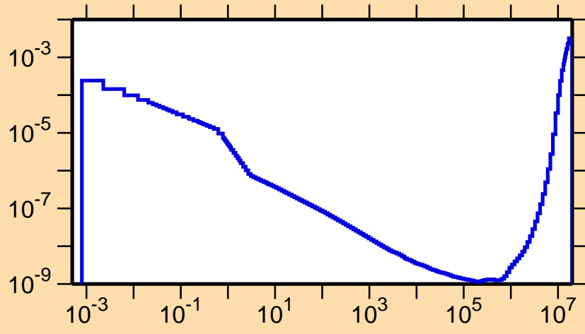
\sigma vs. E for ^{175}\text{Lu}(n,\alpha)
