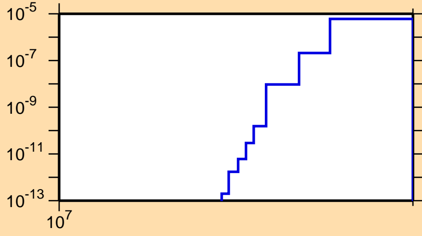
\sigma vs. E for ^{175}\text{Lu}(n,\text{nd})
