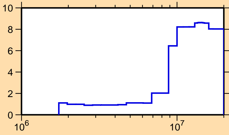
\Delta\sigma/\sigma vs. E for ^{175}\text{Lu}(n,\text{inel.})
