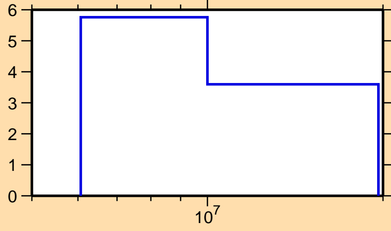
\Delta\sigma/\sigma vs. E for ^{176}\text{Lu}(n,2n)
