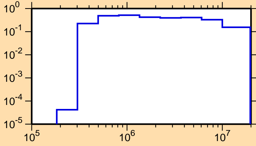
\sigma vs. E for ^{176}\text{Lu}(n,n_4)
