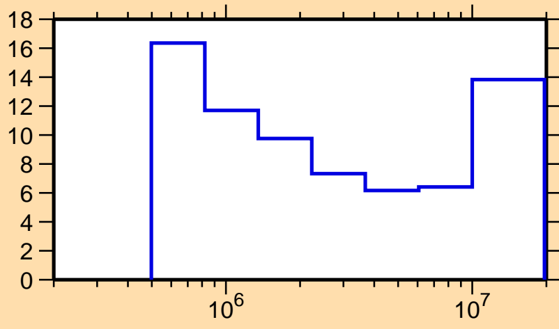
\Delta\sigma/\sigma vs. E for ^{176}\text{Lu}(n,n\text{cont.})
