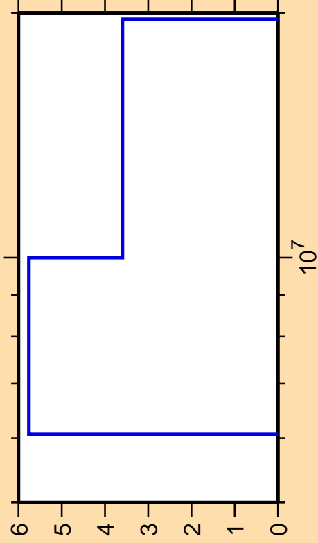
\Delta\sigma/\sigma vs. E for ^{176}\text{Lu}(n,2n)
