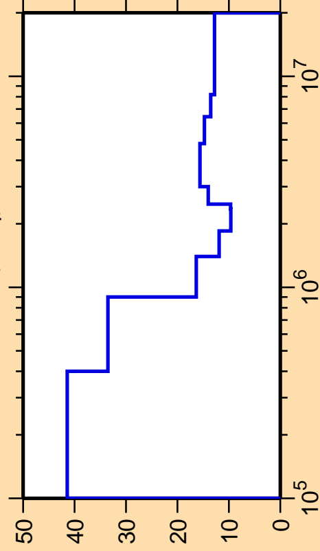
\Delta\sigma/\sigma vs. E for ^{176}\text{Lu}(n,n_4)
