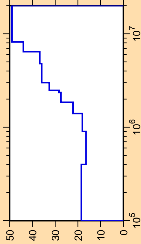
\Delta\sigma/\sigma vs. E for ^{176}\text{Lu}(n,n_2)
