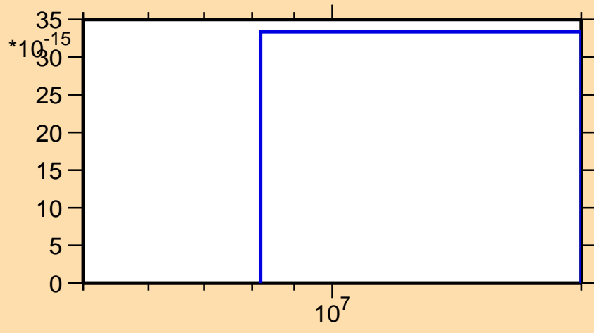
\sigma vs. E for ^{176}\text{Lu}(n,p\alpha)
