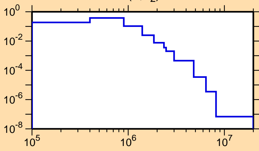
\sigma vs. E for ^{176}\text{Lu}(n,n_2)
