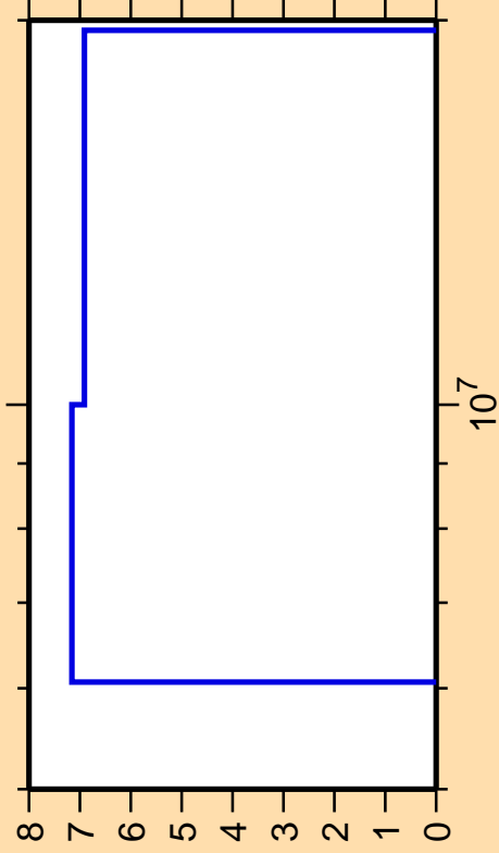
\Delta\sigma/\sigma vs. E for ^{177}\text{Lu}(n,2n)
