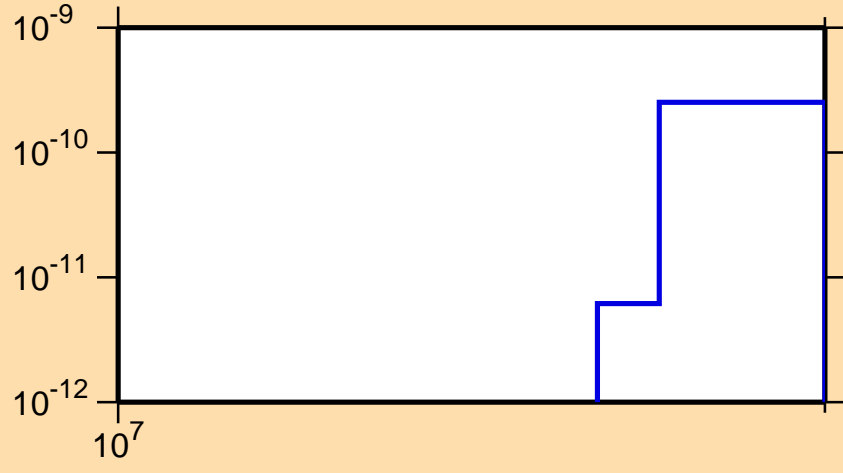
\sigma vs. E for ^{177}\text{Lu}(n,\text{He3})
