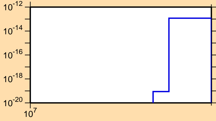
\sigma vs. E for ^{177}\text{Lu} (mt 11)
