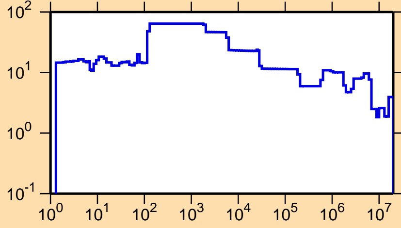
\Delta\sigma/\sigma vs. E for ^{177}\text{Lu}(n, el.)
