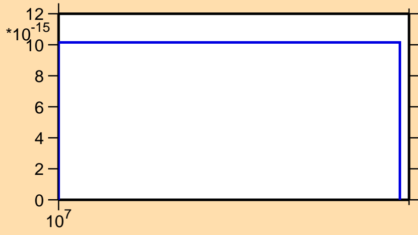
\sigma vs. E for ^{177}\text{Lu}(n,p\alpha)
