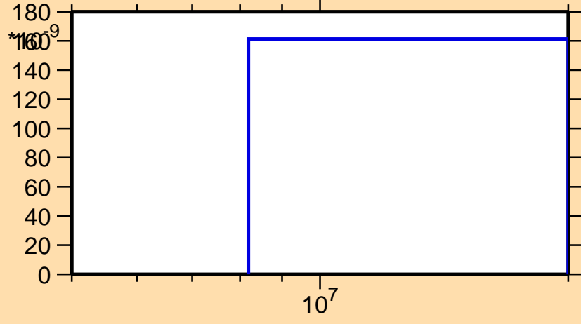
\sigma vs. E for ^{177}\text{Lu}(n,nd)
