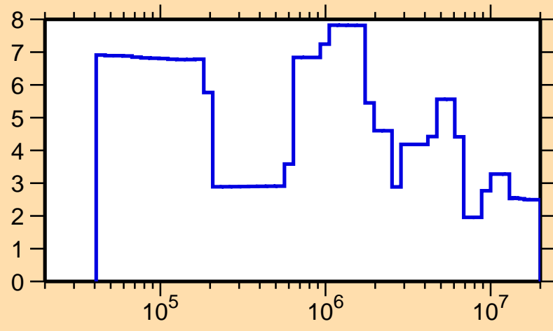
\Delta\sigma/\sigma vs. E for ^{178}\text{Lu}(n,\text{el.})
