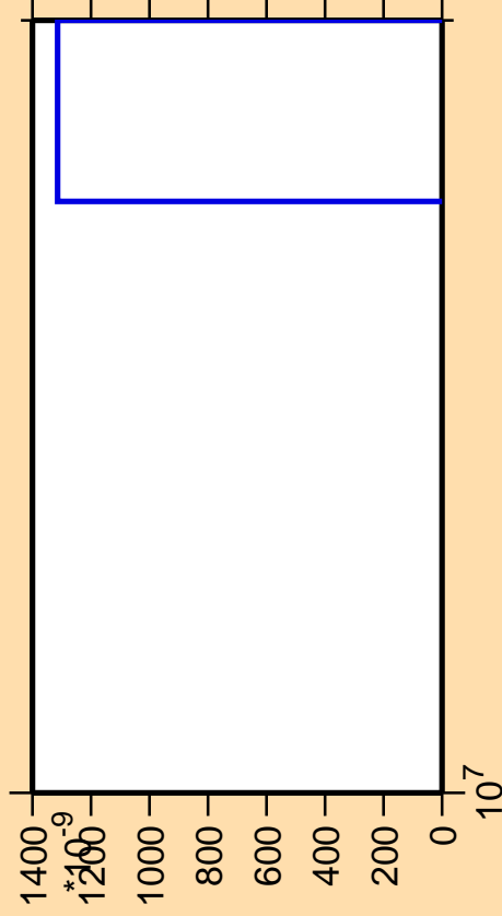
\Delta\sigma/\sigma vs. E for ^{178}\text{Lu} (mt 42)
