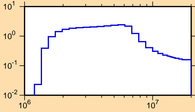
\sigma vs. E for ^{178}\text{Lu}(n,n\text{cont.})
