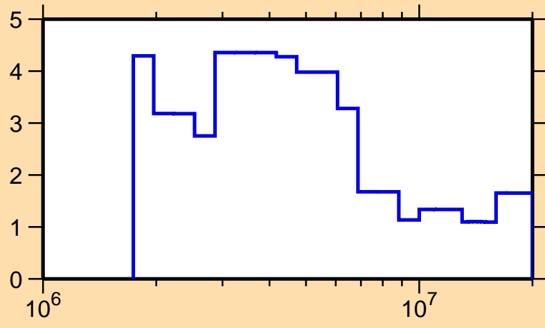
\Delta\sigma/\sigma vs. E for ^{178}\text{Lu}(n,\text{tot.})
