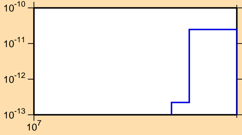
\sigma vs. E for ^{178}\text{Lu}(n,\text{He3})
