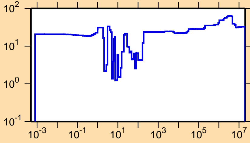
\Delta\sigma/\sigma vs. E for ^{178}\text{Lu}(n,\gamma)
