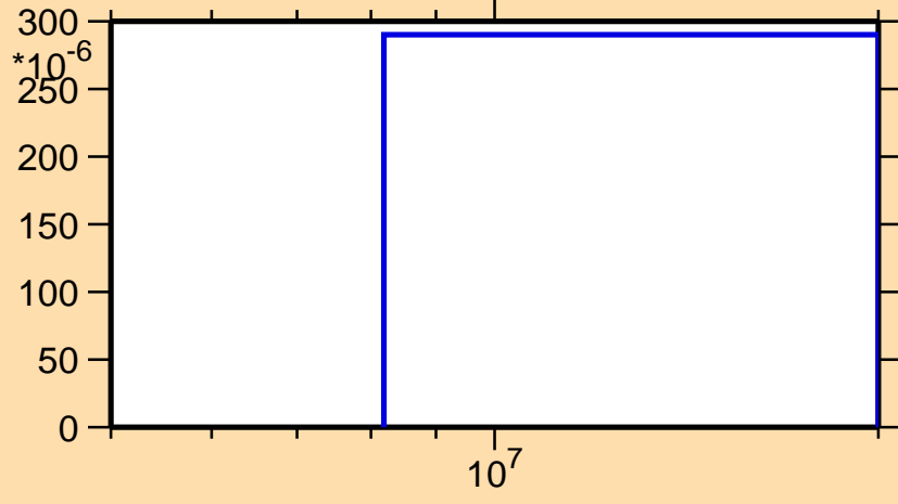
\sigma vs. E for ^{178}\text{Lu}(n,np)
