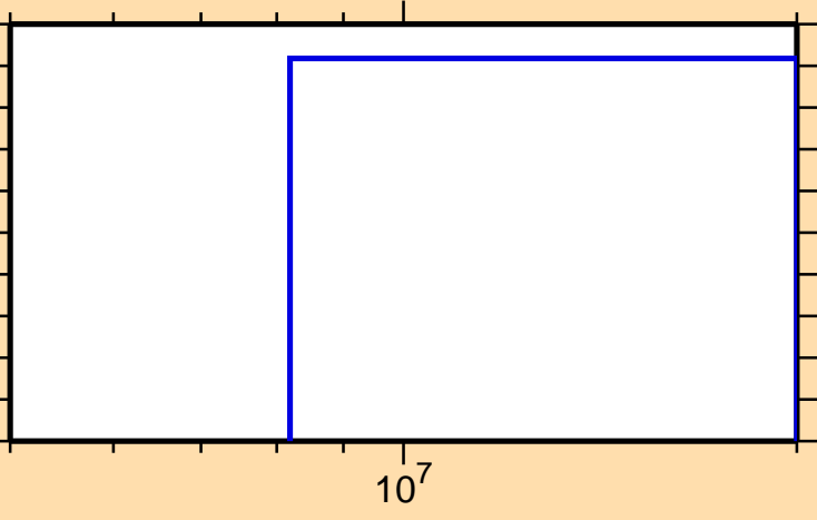
\sigma vs. E for ^{178}\text{Lu}(n,2np)
