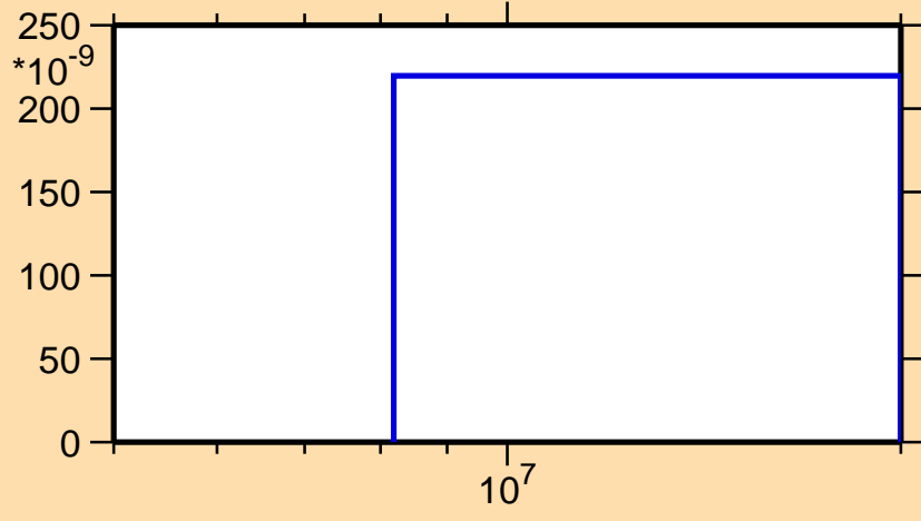
\sigma vs. E for ^{178}\text{Lu}(n,\text{nd})
