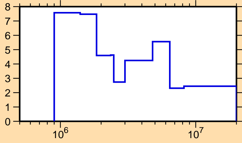
\Delta\sigma/\sigma vs. E for ^{178}\text{Lu}(n, el.)
