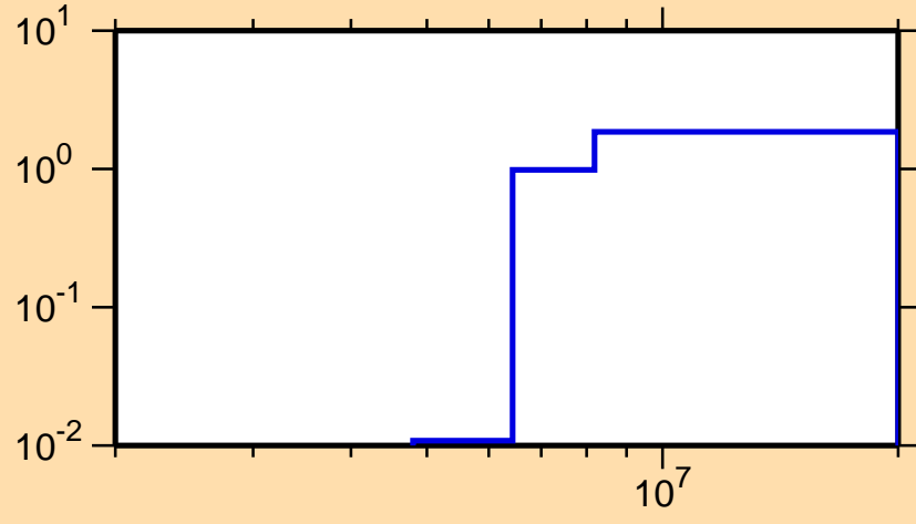
\sigma vs. E for ^{178}\text{Lu}(n,2n)
