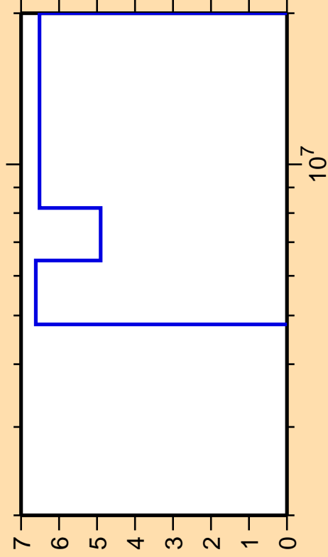
\Delta\sigma/\sigma vs. E for ^{178}\text{Lu}(n,2n)
