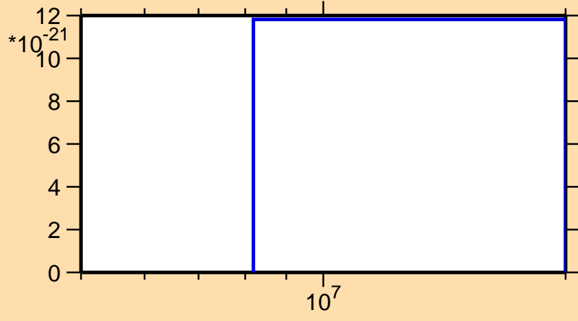
\sigma vs. E for ^{178}\text{Lu} (mt 42)
