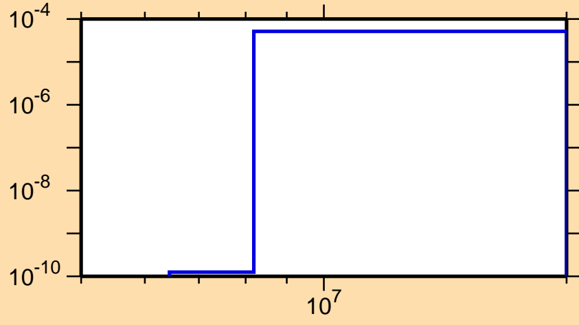
\sigma vs. E for ^{178}\text{Lu}(n,n\alpha)
