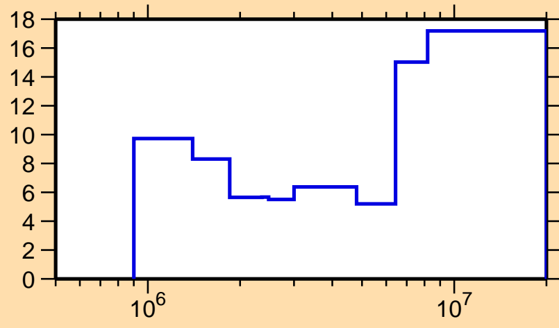
\Delta\sigma/\sigma vs. E for ^{178}\text{Lu}(n,n\text{cont.})
