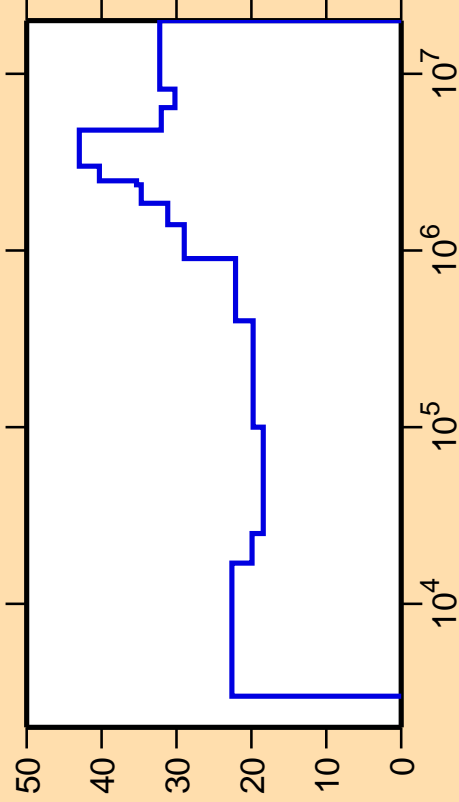
\Delta\sigma/\sigma vs. E for ^{178}\text{Lu}(n,\gamma)
