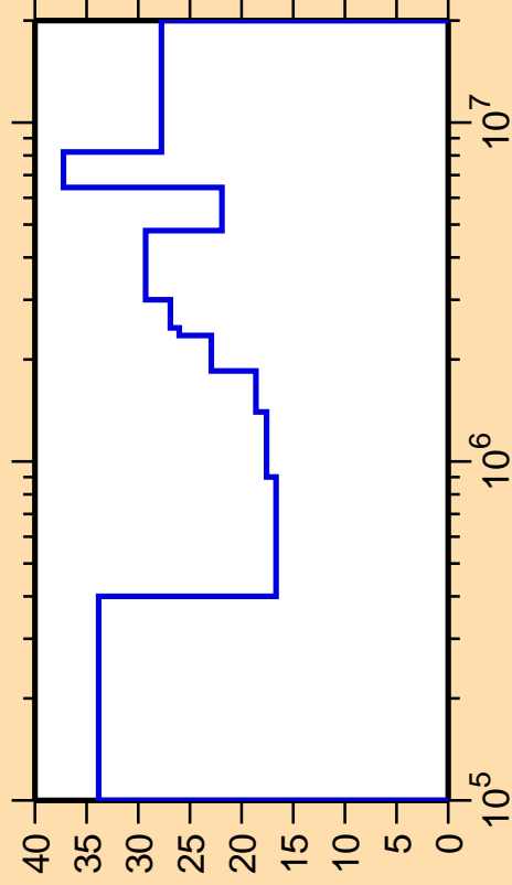
\Delta\sigma/\sigma vs. E for ^{178}\text{Lu}(n,n_2)
