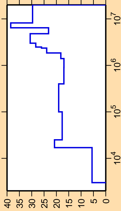
\Delta\sigma/\sigma vs. E for ^{178}\text{Lu}(n,n_1)
