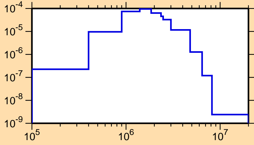
\sigma vs. E for ^{178}\text{Lu}(n,n_2)
