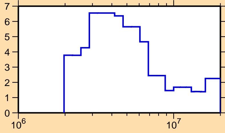
\Delta\sigma/\sigma vs. E for ^{179}\text{Lu}(n,\text{tot.})
