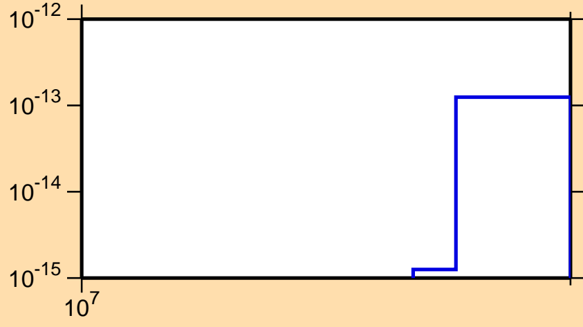
\sigma vs. E for ^{179}\text{Lu}(n,3n\alpha)
