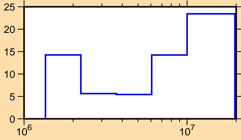
\Delta\sigma/\sigma vs. E for ^{179}\text{Lu}(n,n\text{cont.})
