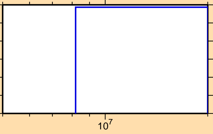
\sigma vs. E for ^{179}\text{Lu}(n,t)
