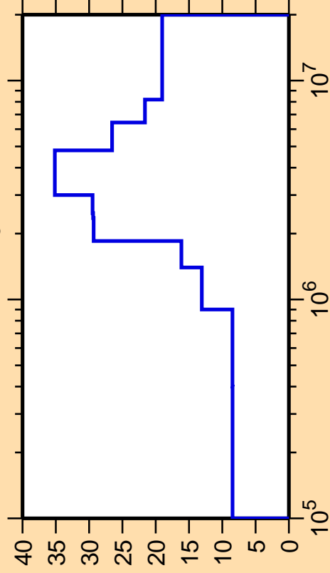
\Delta\sigma/\sigma vs. E for ^{179}\text{Lu}(n,n_3)
