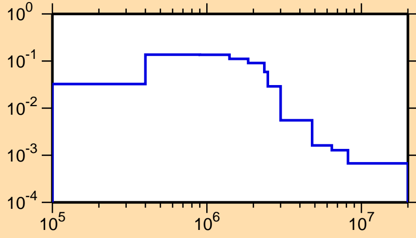
\sigma vs. E for ^{179}\text{Lu}(n,n_3)
