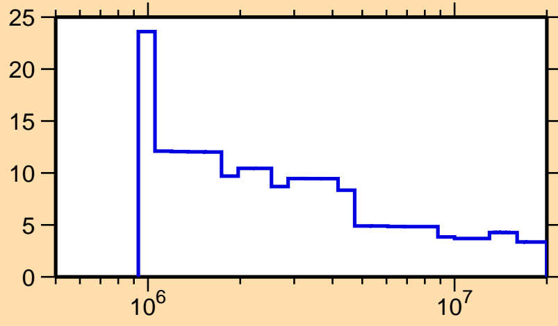
\Delta\sigma/\sigma vs. E for ^{180}\text{Lu}(n,\text{nonel.})
