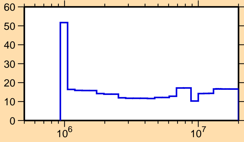
\Delta\sigma/\sigma vs. E for ^{180}\text{Lu}(n,n\text{cont.})
