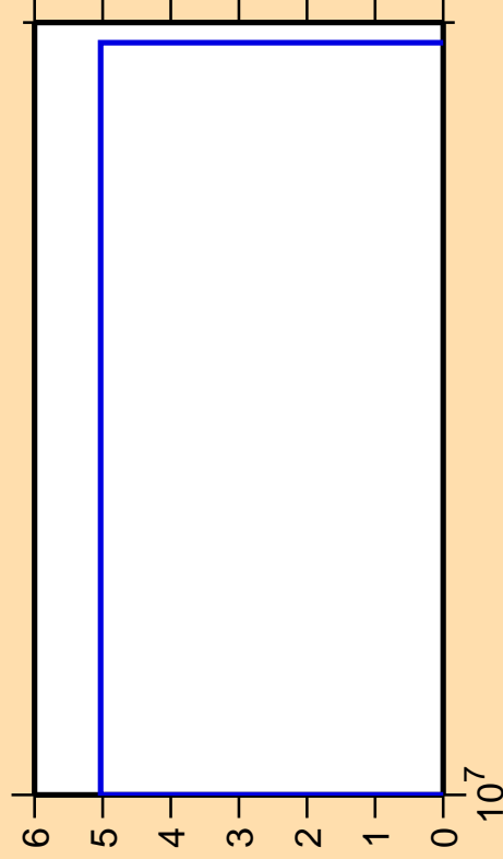
\Delta\sigma/\sigma vs. E for ^{180}\text{Lu}(n,3n)
