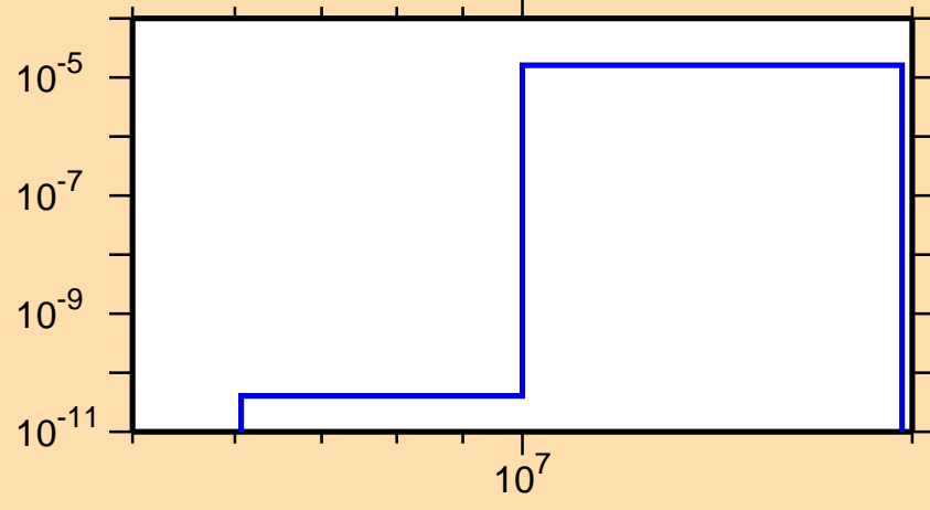
\sigma vs. E for ^{180}\text{Lu}(n,n\alpha)
