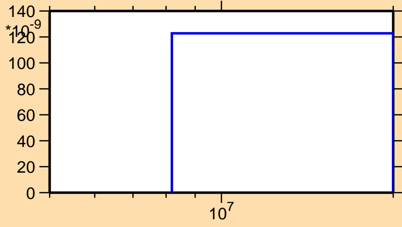
\sigma vs. E for ^{180}\text{Lu}(n,nd)
