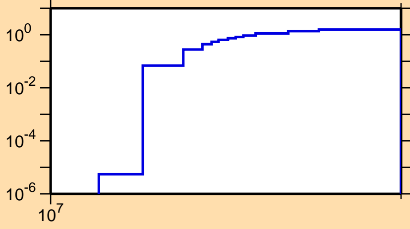
\sigma vs. E for ^{181}\text{Lu}(n,3n)
