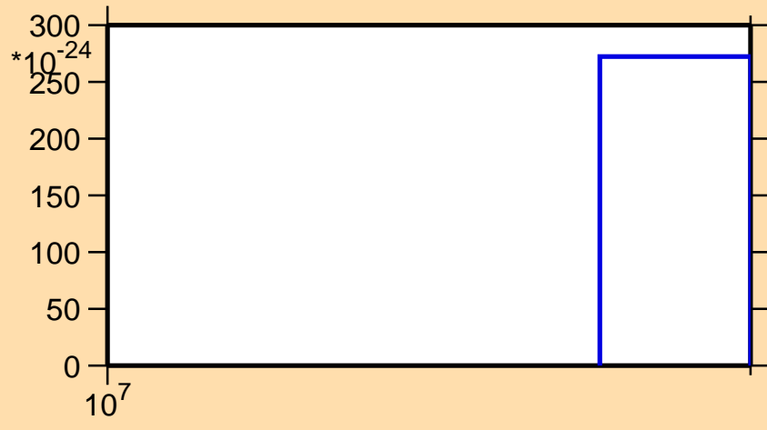
\sigma vs. E for ^{181}\text{Lu} (mt 42)
