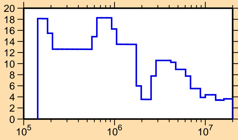
\Delta\sigma/\sigma vs. E for ^{181}\text{Lu}(n, tot.)
