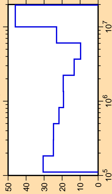
\Delta\sigma/\sigma vs. E for ^{181}\text{Lu}(n,\text{ncont.})
