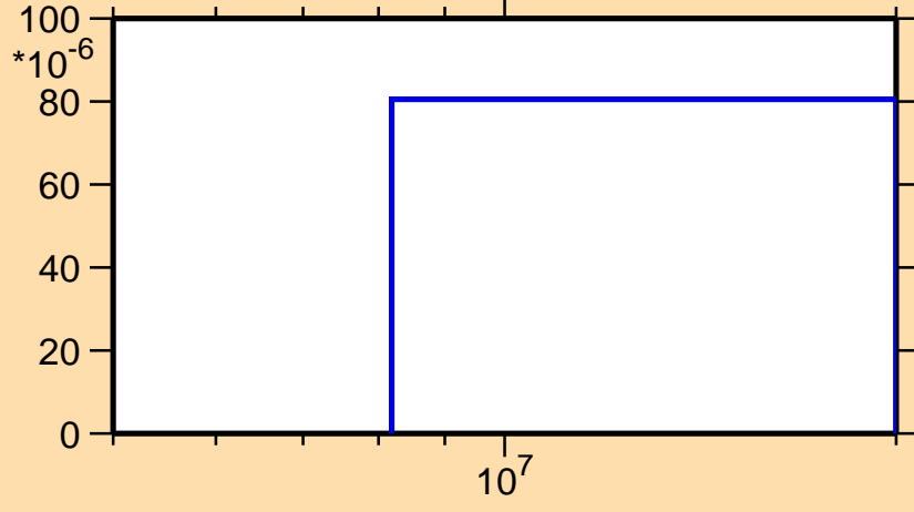
\sigma vs. E for ^{182}\text{Lu}(n,d)
