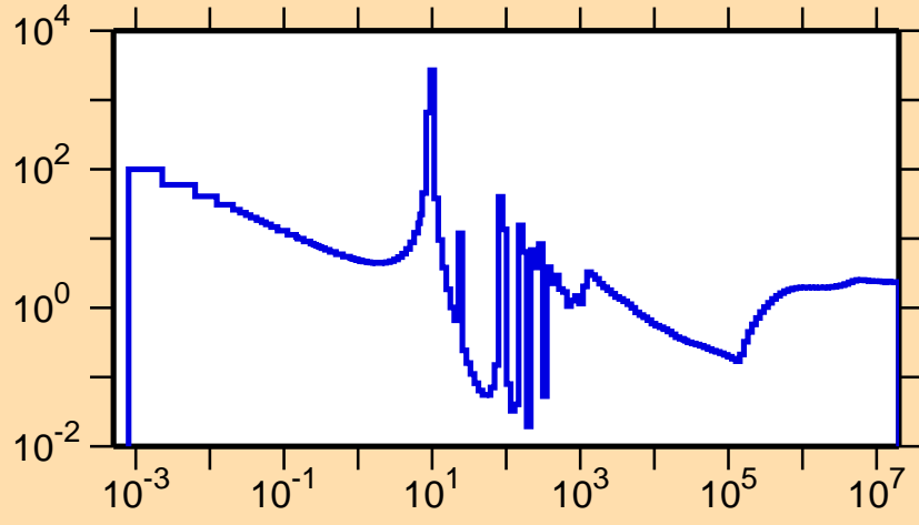
\sigma vs. E for ^{183}\text{Lu}(n,\text{nonel.})
