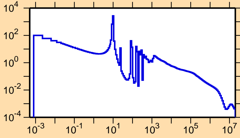
\sigma vs. E for ^{183}\text{Lu}(n,\gamma)
