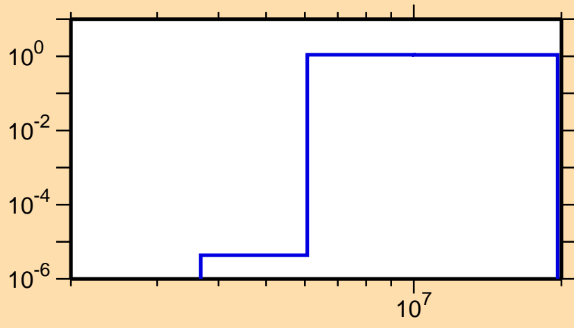
\sigma vs. E for ^{183}\text{Lu}(n,2n)
