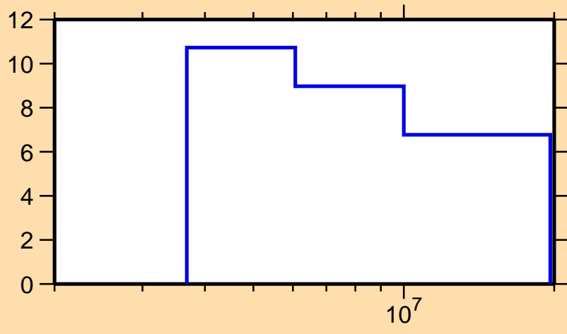
\Delta\sigma/\sigma vs. E for ^{183}\text{Lu}(n,\text{nonel.})
