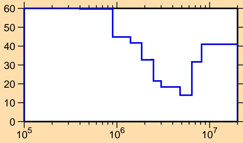
\Delta\sigma/\sigma vs. E for ^{183}\text{Lu}(n,n\text{cont.})
