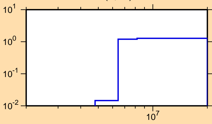
\sigma vs. E for ^{183}\text{Lu}(n,2n)
