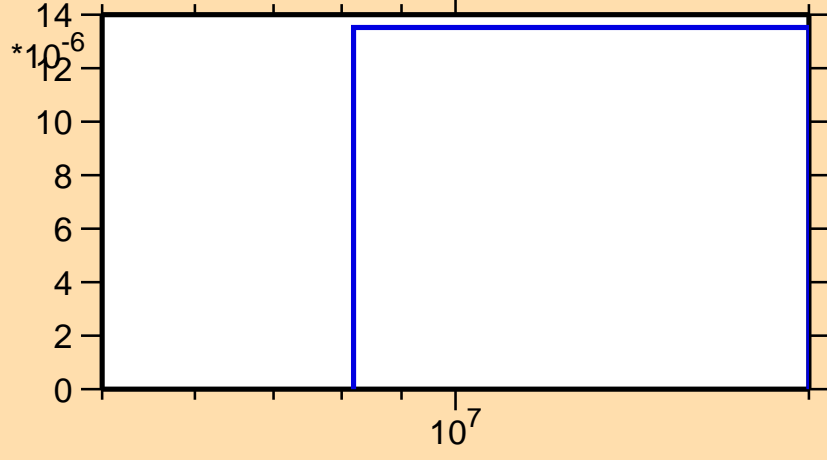
\sigma vs. E for ^{183}\text{Lu}(n,t)
