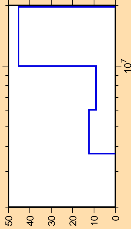
\Delta\sigma/\sigma vs. E for ^{184}\text{Lu}(n,2n)
