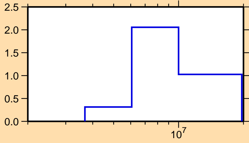
\sigma vs. E for ^{184}\text{Lu}(n,2n)
