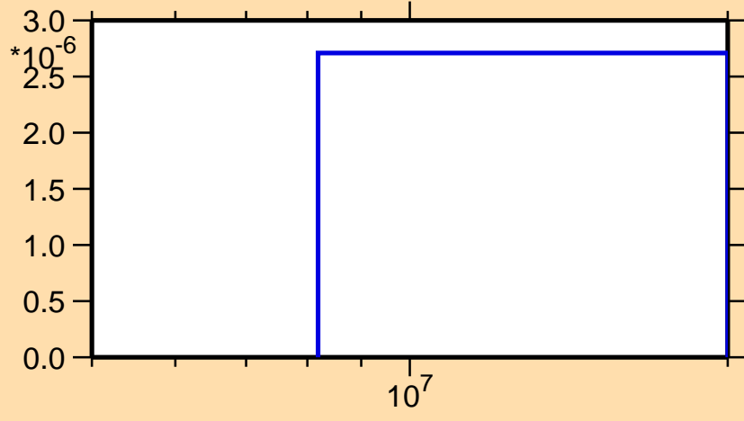
\sigma vs. E for ^{184}\text{Lu}(n,n\alpha)
