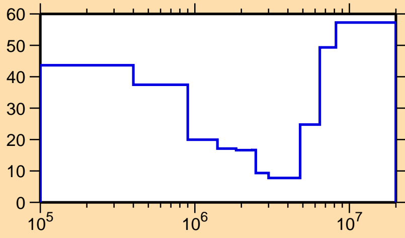
\Delta\sigma/\sigma vs. E for ^{184}\text{Lu}(n,n\text{cont.})
