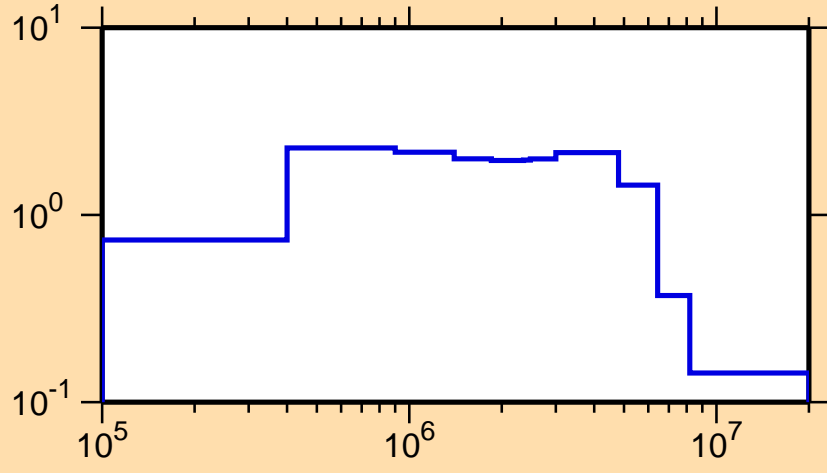
\sigma vs. E for ^{184}\text{Lu}(n,n\text{cont.})
