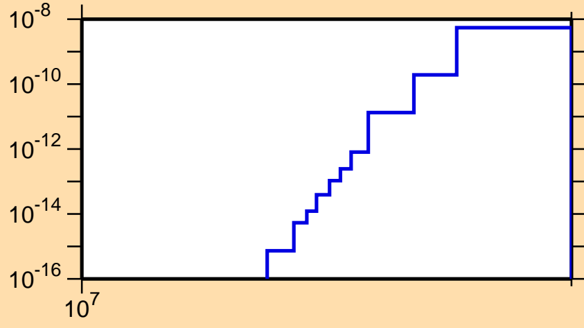
\sigma vs. E for ^{185}\text{Lu}(n,2n\alpha)
