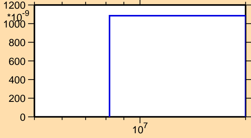
\sigma vs. E for ^{185}\text{Lu}(n,n\alpha)
