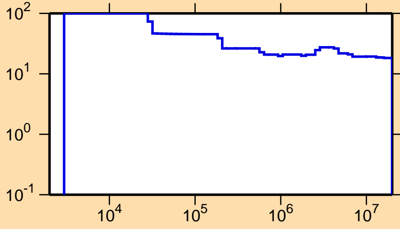
\Delta\sigma/\sigma vs. E for ^{246}\text{Md}(n,n\text{onel.})
