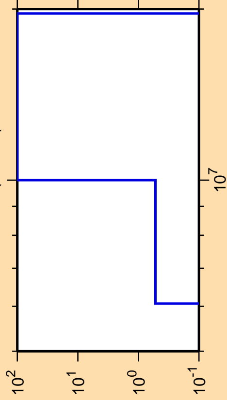
\Delta\sigma/\sigma vs. E for ^{246}\text{Md} (mt 45)
