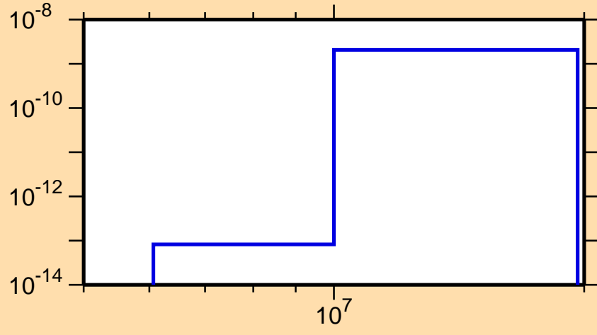
\sigma vs. E for ^{246}\text{Md}(\text{mt117})
