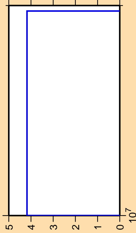
\Delta\sigma/\sigma vs. E for ^{246}\text{Md}(n,\text{pt})
