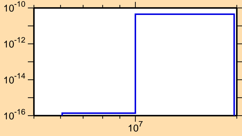
\sigma vs. E for ^{246}\text{Md} (mt 45)
