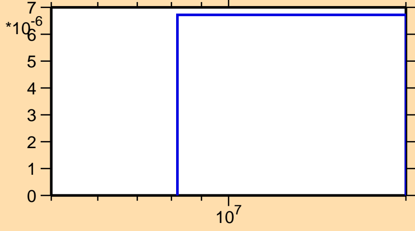
\sigma vs. E for ^{246}\text{Md}(n,nd)
