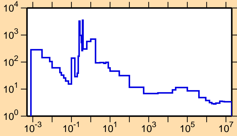
\sigma vs. E for ^{246}\text{Md}(n,f)
