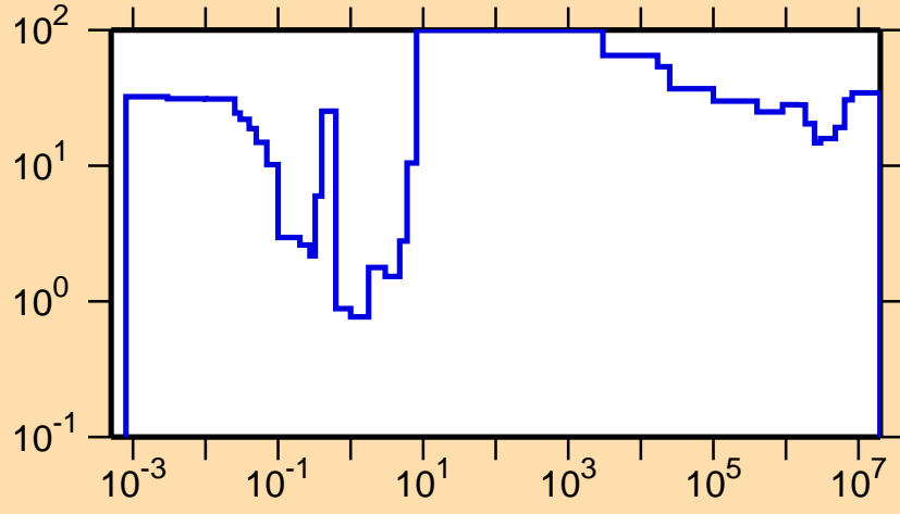
\Delta\sigma/\sigma vs. E for ^{246}\text{Md}(n,tot.)
