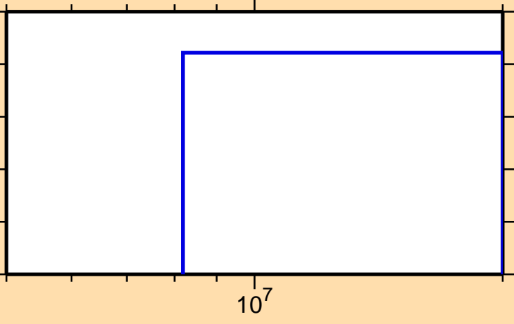
\sigma vs. E for ^{246}\text{Md}(n,3n)
