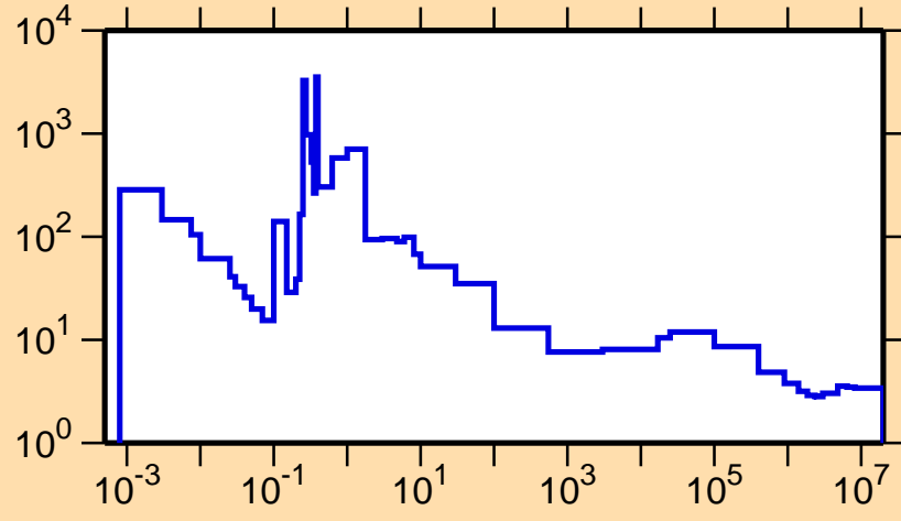
\sigma vs. E for ^{246}\text{Md}(n,\text{nonel.})
