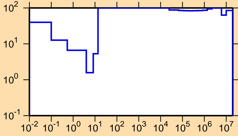
\Delta\sigma/\sigma vs. E for ^{247}\text{Md}(n,\gamma)
