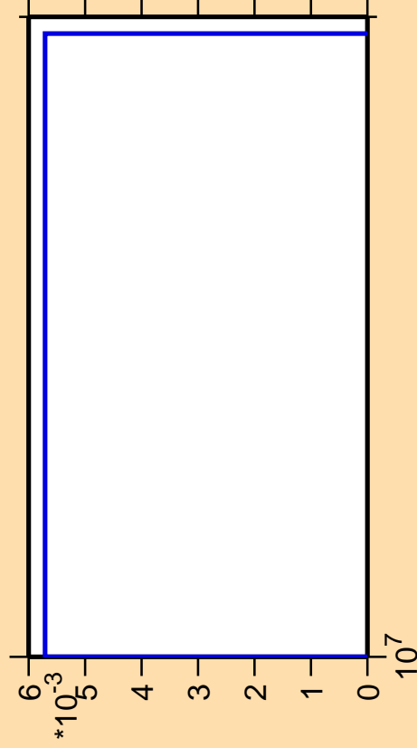
\Delta\sigma/\sigma vs. E for ^{247}\text{Md}(n,\text{pd})
