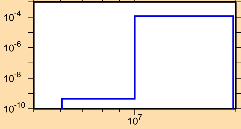
\sigma vs. E for ^{247}\text{Md}(n,t)
