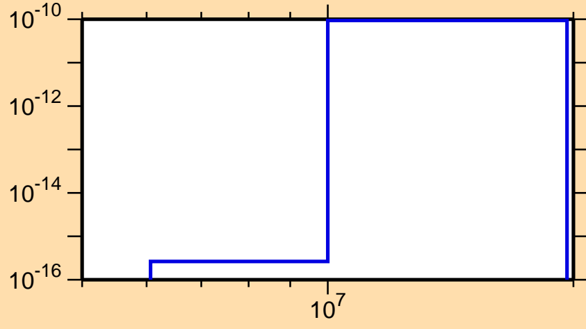
\sigma vs. E for ^{247}\text{Md} (mt 45)
