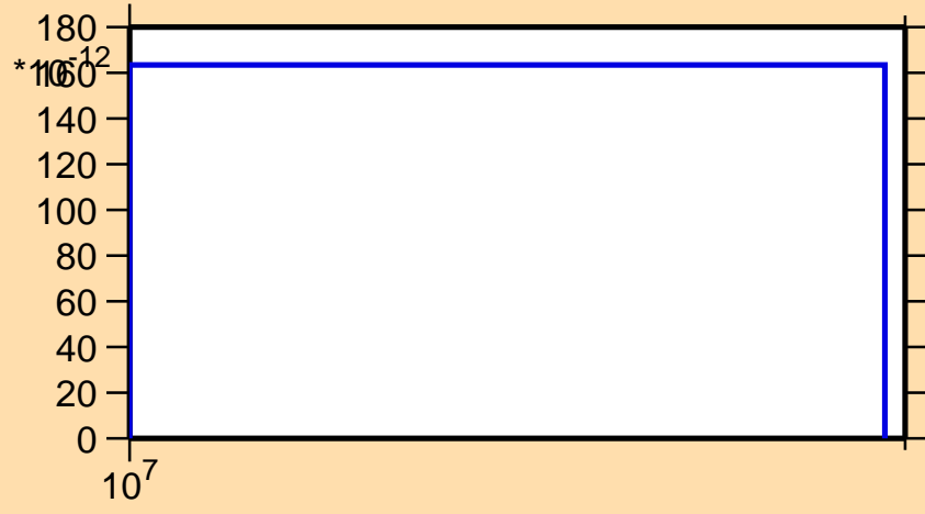
\sigma vs. E for ^{247}\text{Md}(n,\text{nd})
