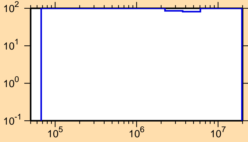
\Delta\sigma/\sigma vs. E for ^{247}\text{Md}(n,n\text{cont.})
