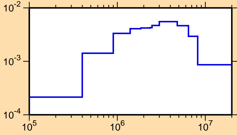
\sigma vs. E for ^{247}\text{Md}(n,n\alpha)
