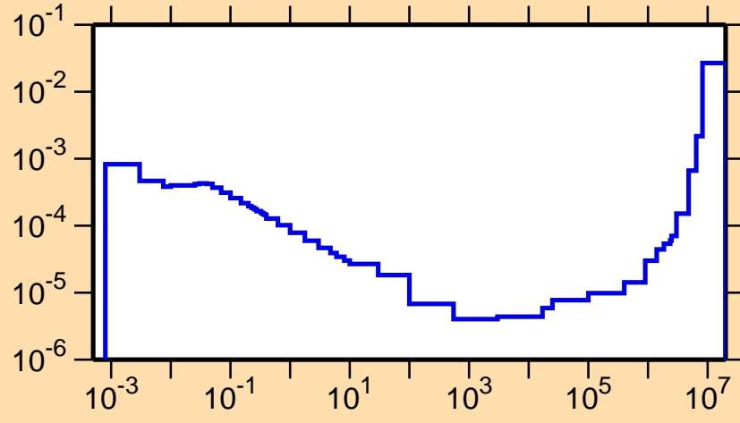
\sigma vs. E for ^{247}\text{Md}(n,p)
