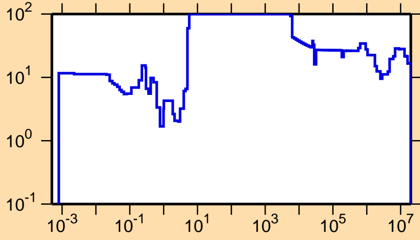
\Delta\sigma/\sigma vs. E for ^{248}\text{Md}(n,\text{tot.})
