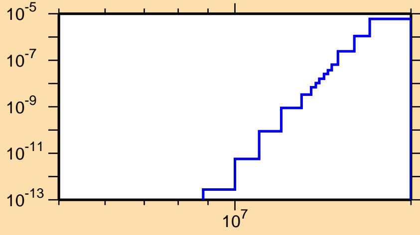
\sigma vs. E for ^{248}\text{Md}(n,\text{He3})
