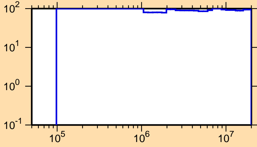
\Delta\sigma/\sigma vs. E for ^{248}\text{Md}(n,n_1)
