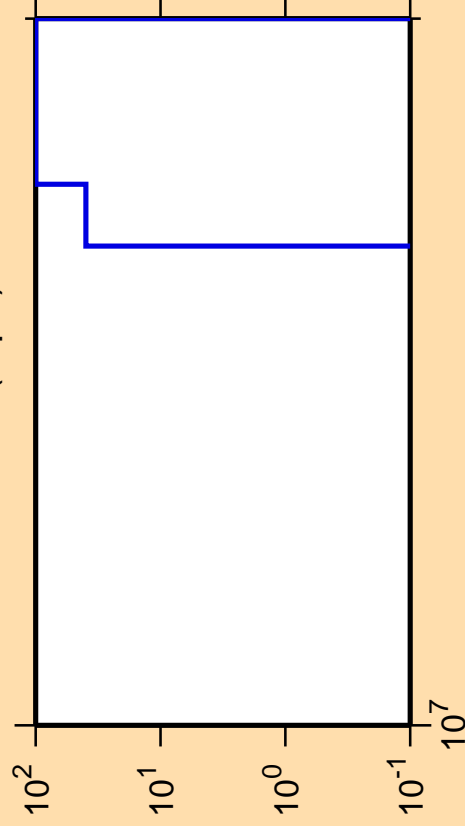
\Delta\sigma/\sigma vs. E for ^{248}\text{Md}(n,\text{pd})
