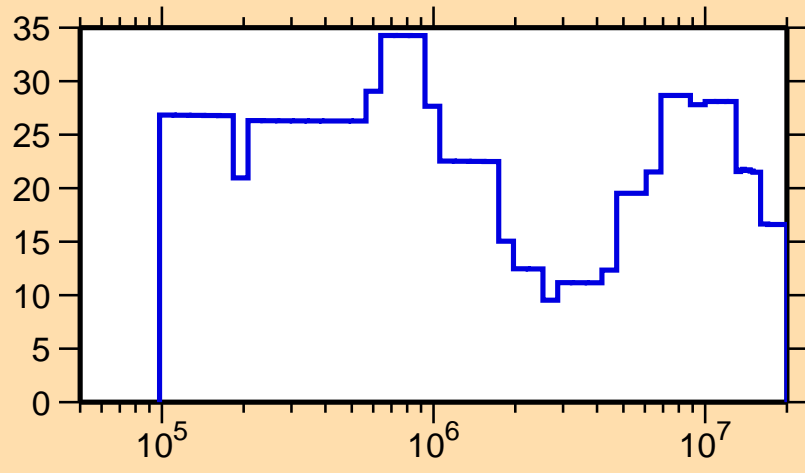
\Delta\sigma/\sigma vs. E for ^{248}\text{Md}(n,\text{tot.})
