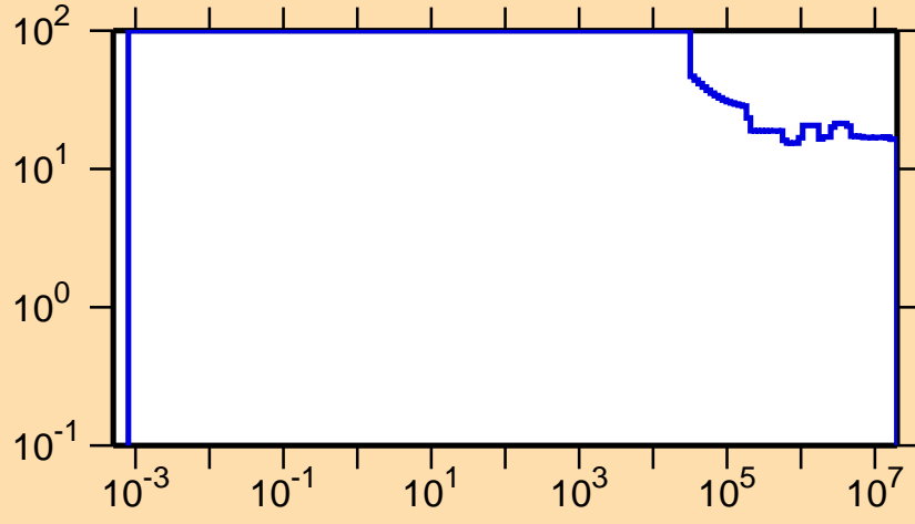
\Delta\sigma/\sigma vs. E for ^{248}\text{Md}(n,\text{nonel.})
