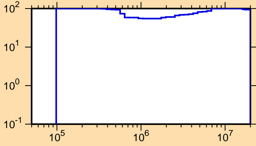
\Delta\sigma/\sigma vs. E for ^{248}\text{Md}(n,n\text{cont.})
