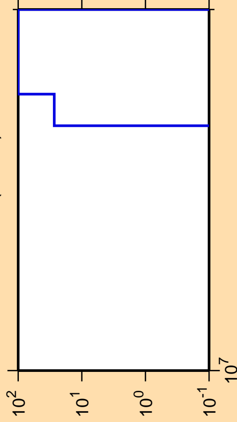
\Delta\sigma/\sigma vs. E for ^{248}\text{Md} (mt 34)
