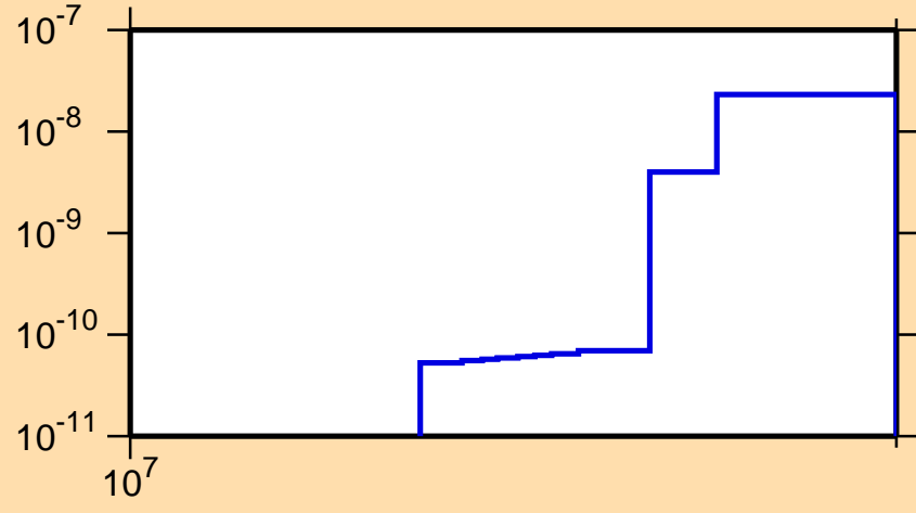
\sigma vs. E for ^{248}\text{Md}(n,3n\alpha)
