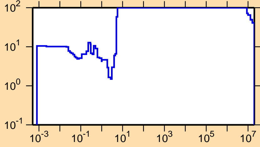
\Delta\sigma/\sigma vs. E for ^{248}\text{Md}(n,f)
