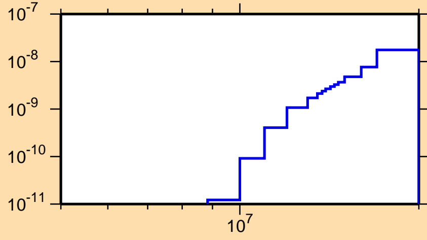
\sigma vs. E for ^{248}\text{Md}(\text{mt117})
