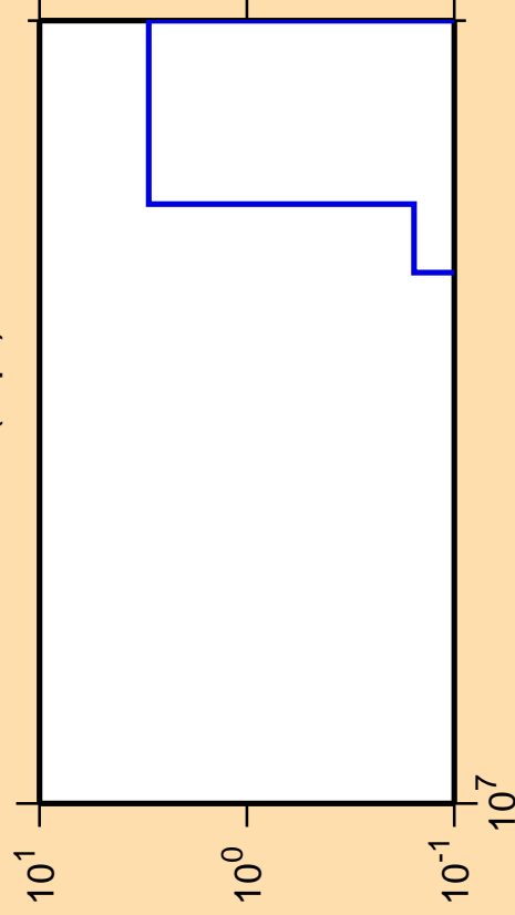
\Delta\sigma/\sigma vs. E for ^{248}\text{Md}(n,\text{pt})
