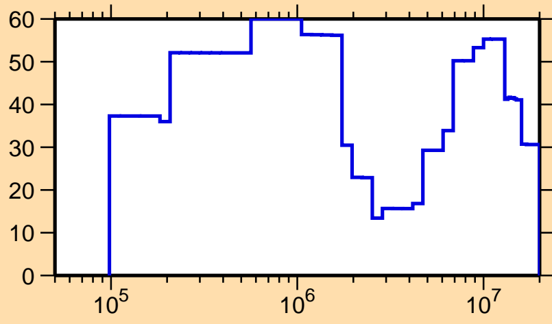
\Delta\sigma/\sigma vs. E for ^{248}\text{Md}(n,\text{el.})
