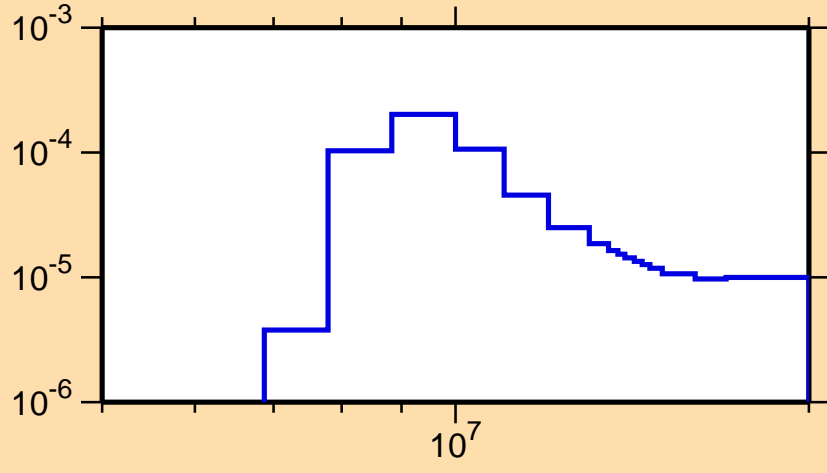
\sigma vs. E for ^{248}\text{Md}(n,2n\alpha)
