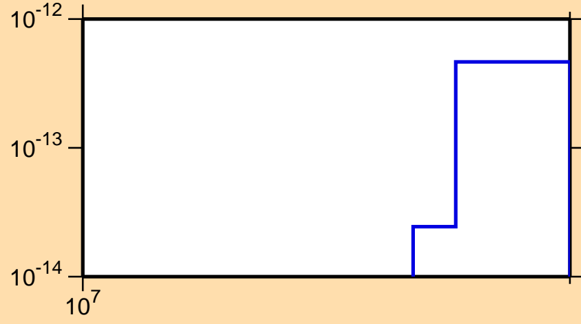
\sigma vs. E for ^{248}\text{Md}(n,\text{pt})
