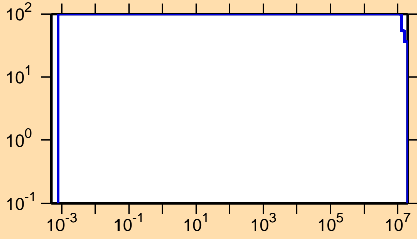
\Delta\sigma/\sigma vs. E for ^{248}\text{Md}(n,p)
