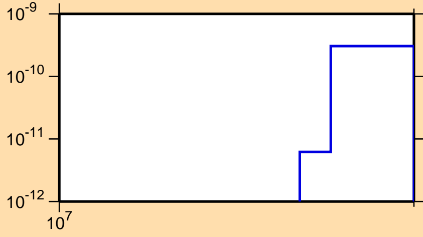
\sigma vs. E for ^{248}\text{Md} (mt 34)
