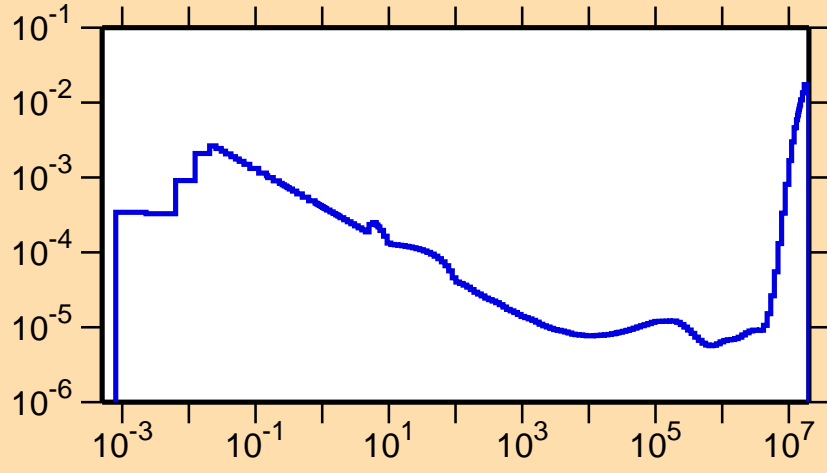
\sigma vs. E for ^{248}\text{Md}(n,\alpha)
