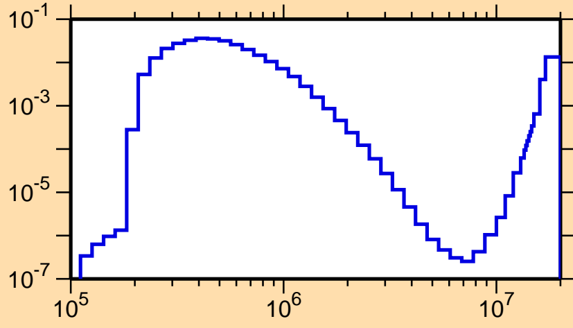
\sigma vs. E for ^{248}\text{Md}(n,n\alpha)
