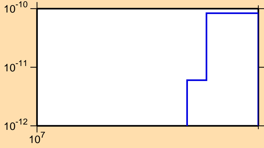
\sigma vs. E for ^{248}\text{Md}(n,\text{pd})
