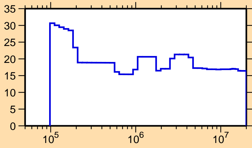
\Delta\sigma/\sigma vs. E for ^{248}\text{Md}(n,\text{nonel.})
