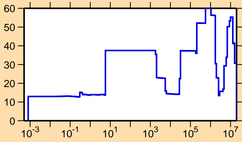
\Delta\sigma/\sigma vs. E for ^{248}\text{Md}(n,el.)
