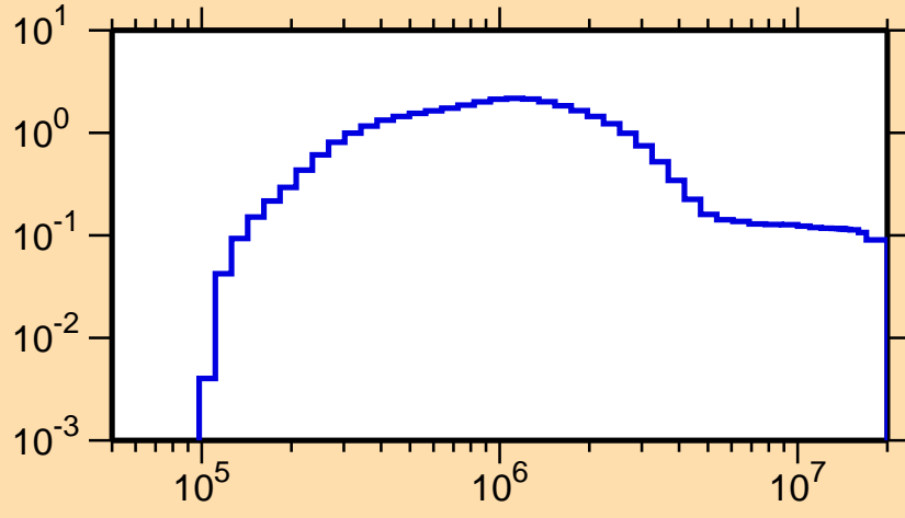
\sigma vs. E for ^{248}\text{Md}(n,n\text{cont.})
