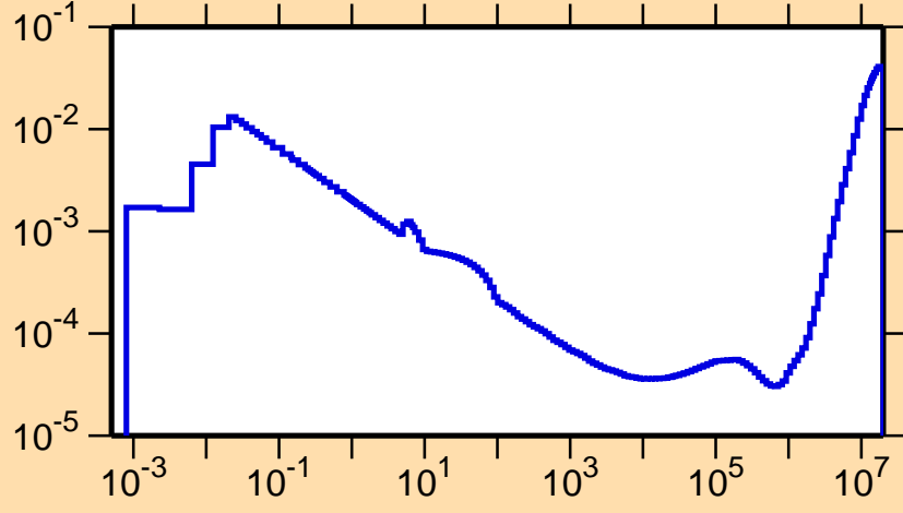
\sigma vs. E for ^{248}\text{Md}(n,p)
