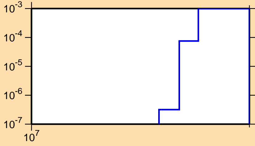
\sigma vs. E for ^{248}\text{Md}(n,3n)
