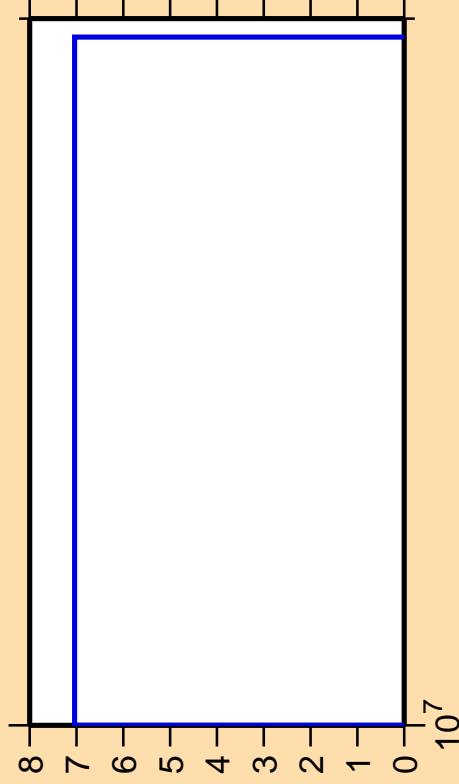
\Delta\sigma/\sigma vs. E for ^{248}\text{Md}(n,\text{pd})
