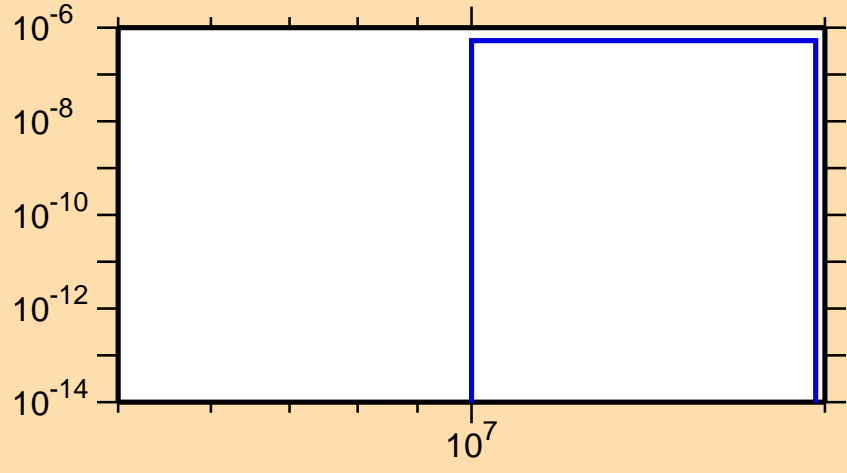
\sigma vs. E for ^{248}\text{Md}(n,nd)
