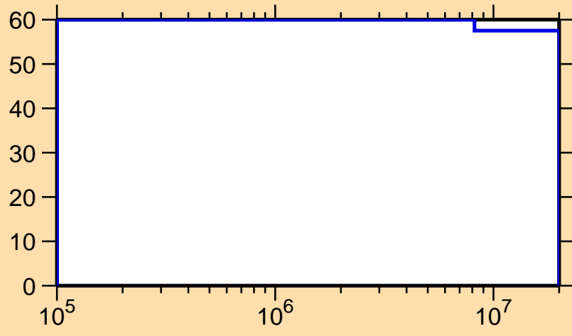
\Delta\sigma/\sigma vs. E for ^{248}\text{Md}(n,f)
