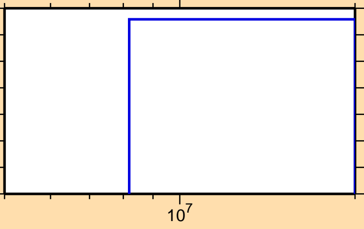
\sigma vs. E for ^{248}\text{Md}(n,\text{He3})
