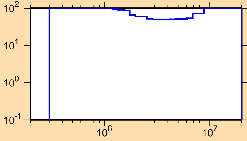
\Delta\sigma/\sigma vs. E for ^{249}\text{Md}(n,n\text{cont.})
