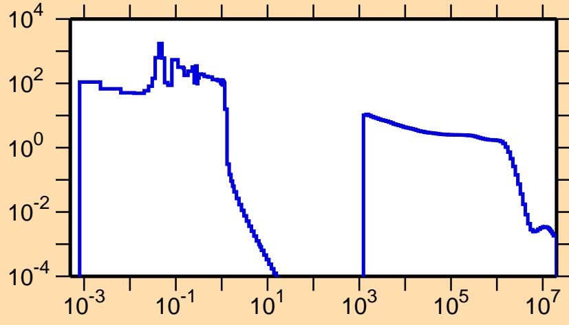
\sigma vs. E for ^{249}\text{Md}(n,\gamma)
