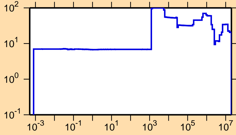
\Delta\sigma/\sigma vs. E for ^{249}\text{Md}(n,el.)
