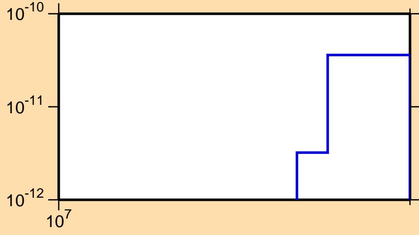
\sigma vs. E for ^{249}\text{Md}(n,\text{pd})
