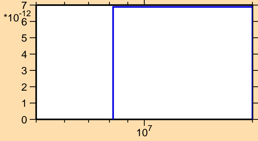
\sigma vs. E for ^{249}\text{Md} (mt 45)
