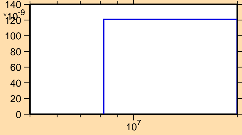
\sigma vs. E for ^{249}\text{Md}(n,nd)
