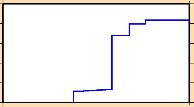
\sigma vs. E for ^{249}\text{Md}(n,3n\alpha)
