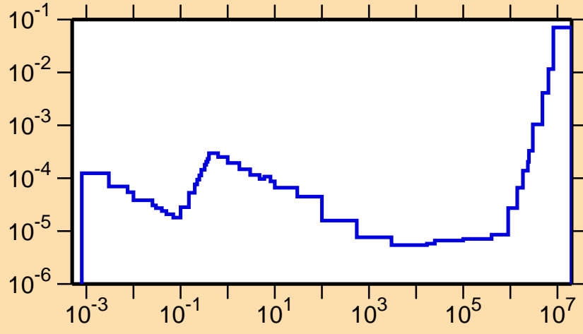
\sigma vs. E for ^{250}\text{Md}(n,p)
