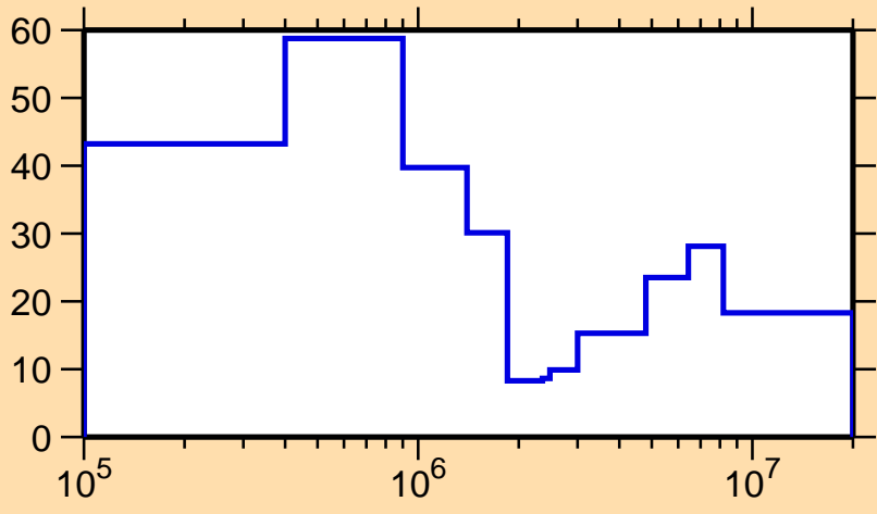
\Delta\sigma/\sigma vs. E for ^{250}\text{Md}(n, el.)
