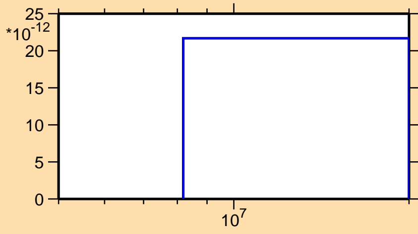
\sigma vs. E for ^{250}\text{Md}(\text{mt } 34)
