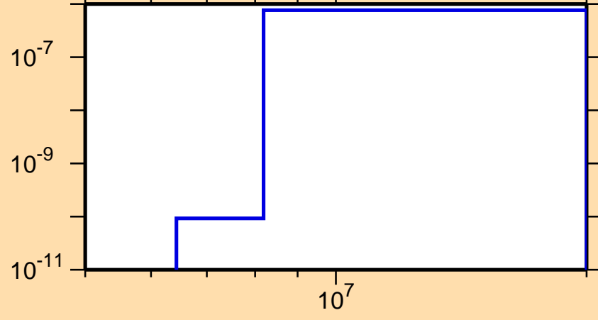
\sigma vs. E for ^{250}\text{Md}(n,t)
