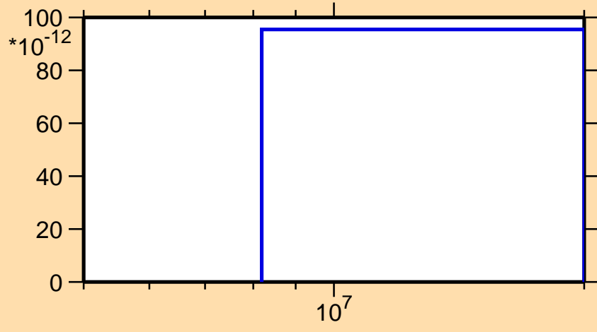
\sigma vs. E for ^{250}\text{Md}(n,\text{nd})
