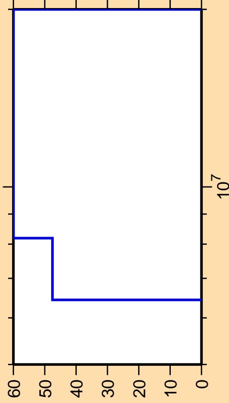
\Delta\sigma/\sigma vs. E for ^{250}\text{Md}(n,p\alpha)
