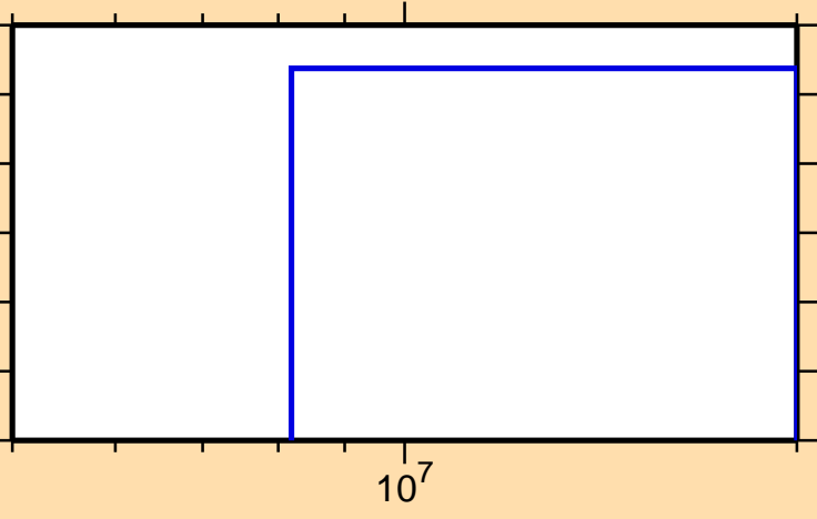
\sigma vs. E for ^{250}\text{Md}(n,nt)
