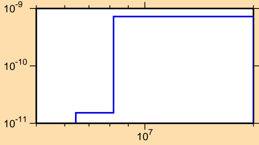
\sigma vs. E for ^{250}\text{Md}(n,p\alpha)
