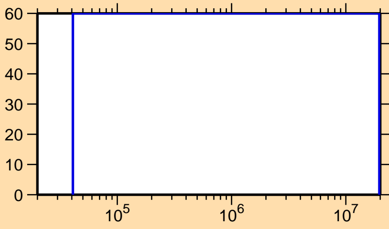
\Delta\sigma/\sigma vs. E for ^{251}\text{Md}(n,n_1)
