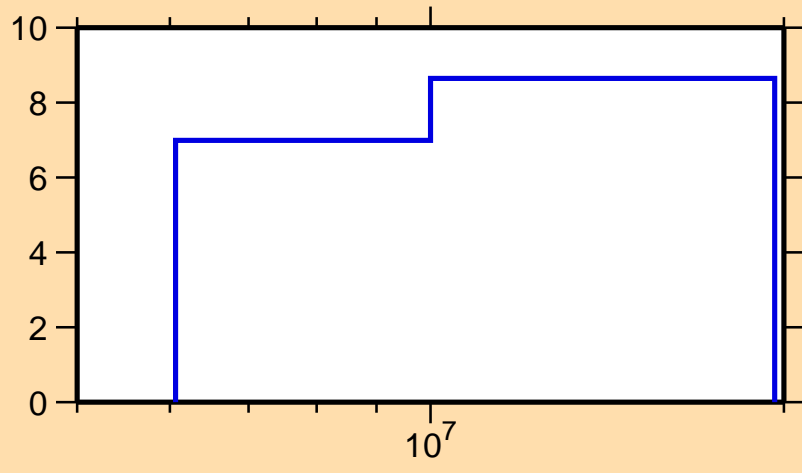
\Delta\sigma/\sigma vs. E for ^{251}\text{Md}(n,\text{nonel.})
