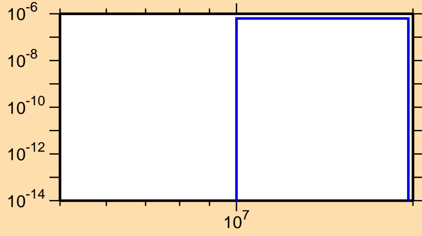
\sigma vs. E for ^{251}\text{Md}(n,2n\alpha)
