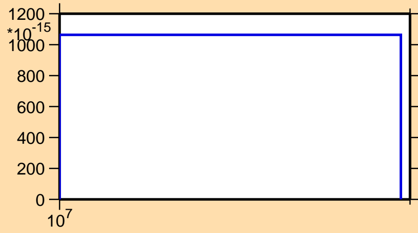
\sigma vs. E for ^{251}\text{Md} (mt 45)
