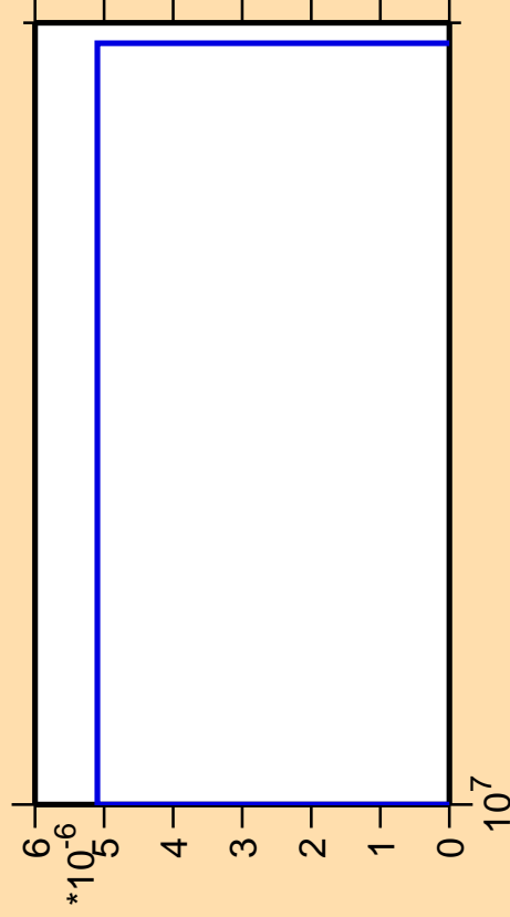
\Delta\sigma/\sigma vs. E for ^{251}\text{Md} (mt 11)
