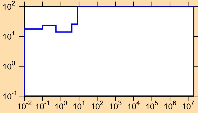
\Delta\sigma/\sigma vs. E for ^{251}\text{Md}(n,f)
