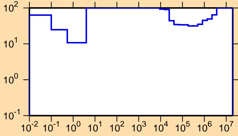
\Delta\sigma/\sigma vs. E for ^{251}\text{Md}(n,\gamma)
