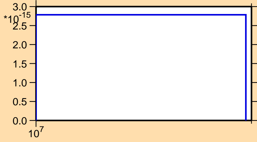
\sigma vs. E for ^{251}\text{Md} (mt 34)
