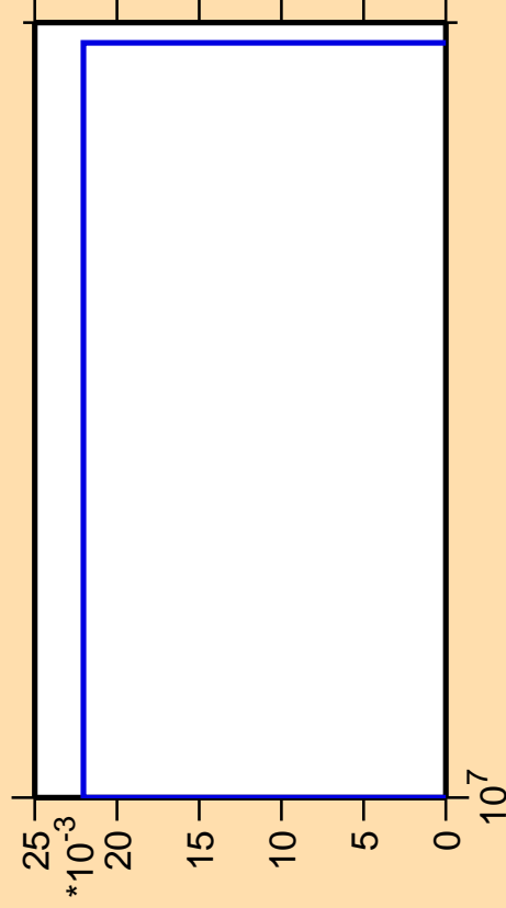
\Delta\sigma/\sigma vs. E for ^{251}\text{Md}(n,3n\alpha)
