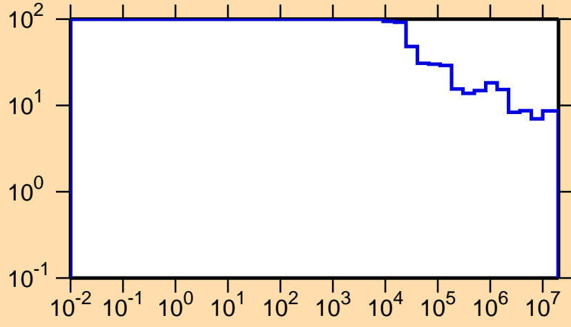
\Delta\sigma/\sigma vs. E for ^{251}\text{Md}(n,\text{nonel.})
