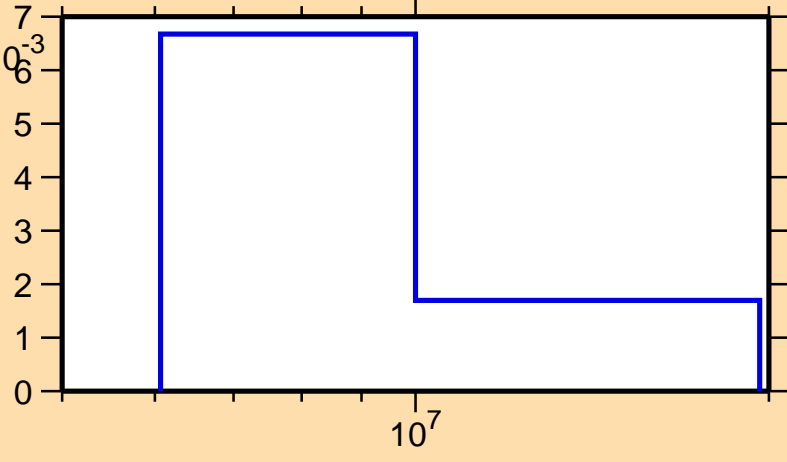
\sigma vs. E for ^{251}\text{Md}(n,2n)
