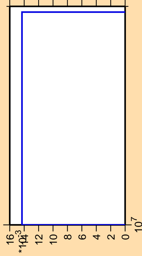
\Delta\sigma/\sigma vs. E for ^{251}\text{Md} (mt 34)
