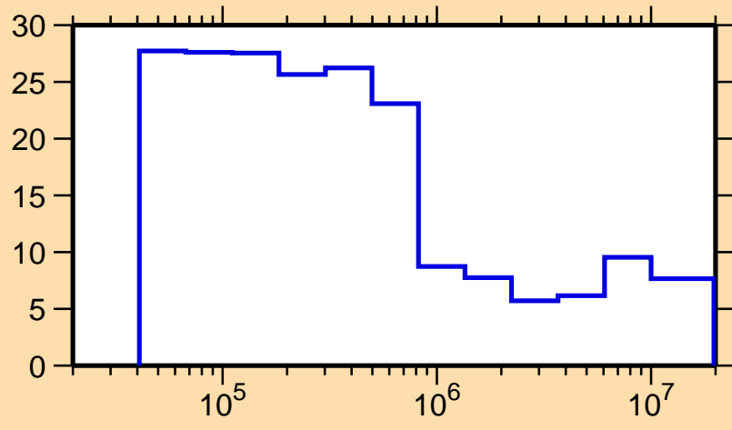
\Delta\sigma/\sigma vs. E for ^{251}\text{Md}(n,\text{tot.})
