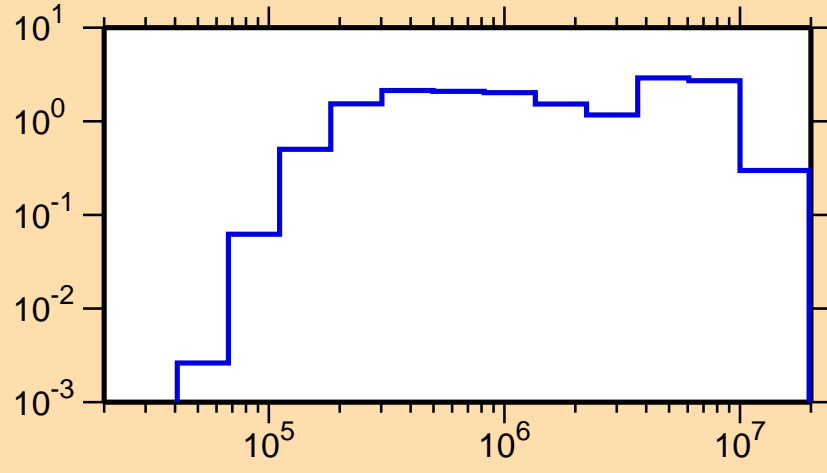
\sigma vs. E for ^{251}\text{Md}(n,\text{inel.})
