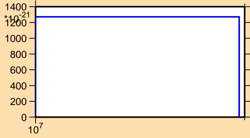
\sigma vs. E for ^{251}\text{Md} (mt 11)
