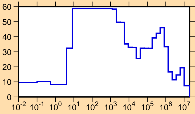
\Delta\sigma/\sigma vs. E for ^{251}\text{Md}(n,\text{el.})
