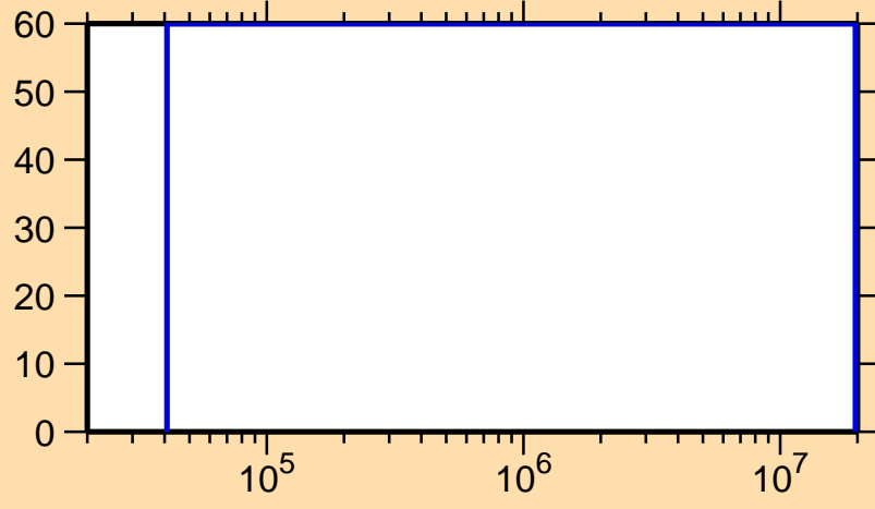
\Delta\sigma/\sigma vs. E for ^{251}\text{Md}(n,n_1)
