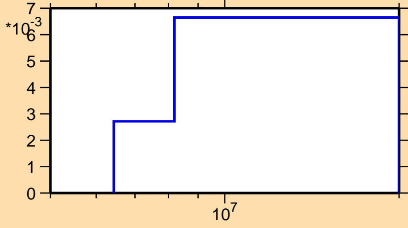
\sigma vs. E for ^{251}\text{Md}(n,2n)
