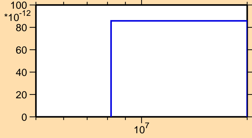
\sigma vs. E for ^{251}\text{Md}(n,nd)
