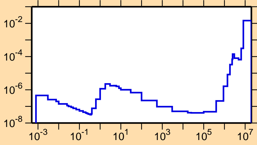
\sigma vs. E for ^{251}\text{Md}(n,p)
