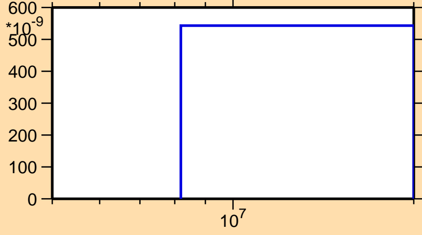
\sigma vs. E for ^{251}\text{Md}(n,3n)
