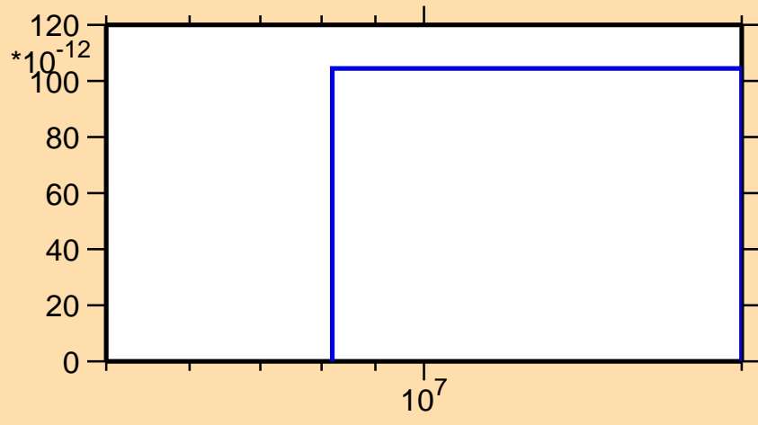
\sigma vs. E for ^{251}\text{Md}(n,2np)
