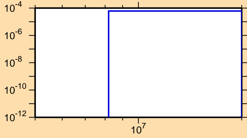
\sigma vs. E for ^{251}\text{Md}(n,t)
