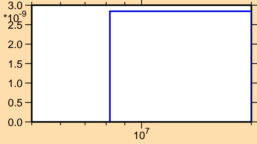
\sigma vs. E for ^{251}\text{Md}(n,p\alpha)
