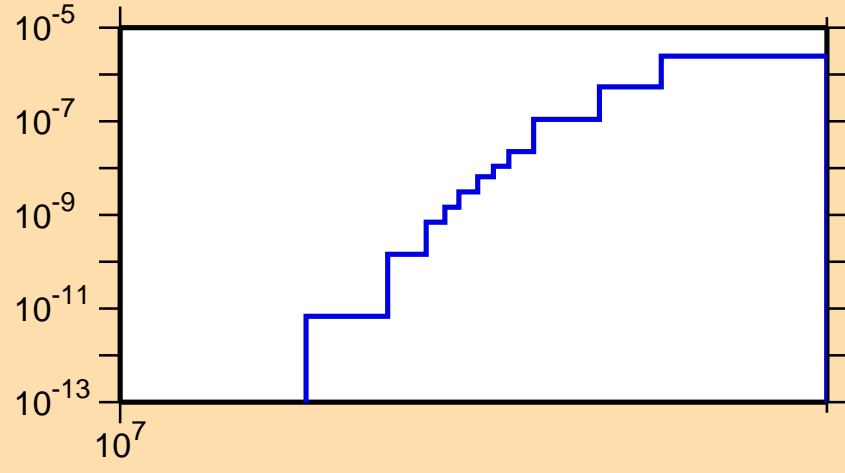
\sigma vs. E for ^{252}\text{Md}(n,2np)
