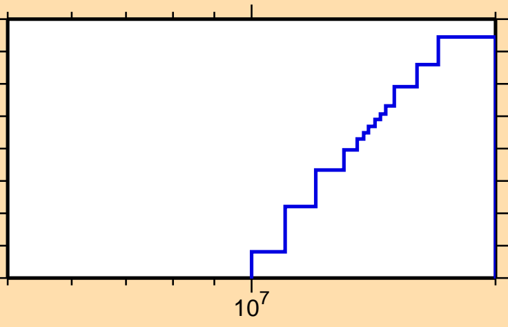
\sigma vs. E for ^{252}\text{Md}(n,\text{He3})
