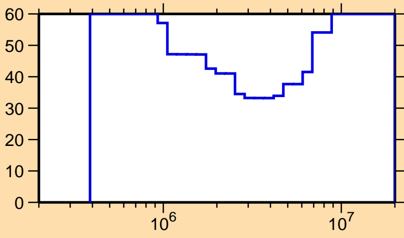
\Delta\sigma/\sigma vs. E for ^{252}\text{Md}(n,n\text{cont.})
