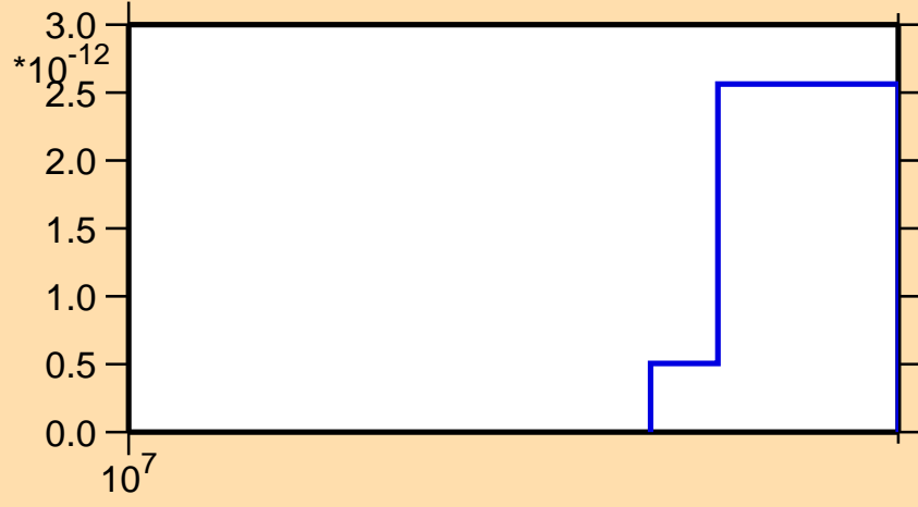
\sigma vs. E for ^{252}\text{Md} (mt 45)
