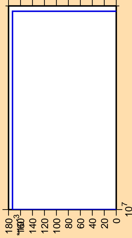
\Delta\sigma/\sigma vs. E for ^{252}\text{Md} (mt 45)
