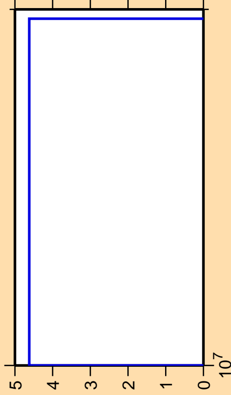
\Delta\sigma/\sigma vs. E for ^{252}\text{Md}(n,3n\alpha)
