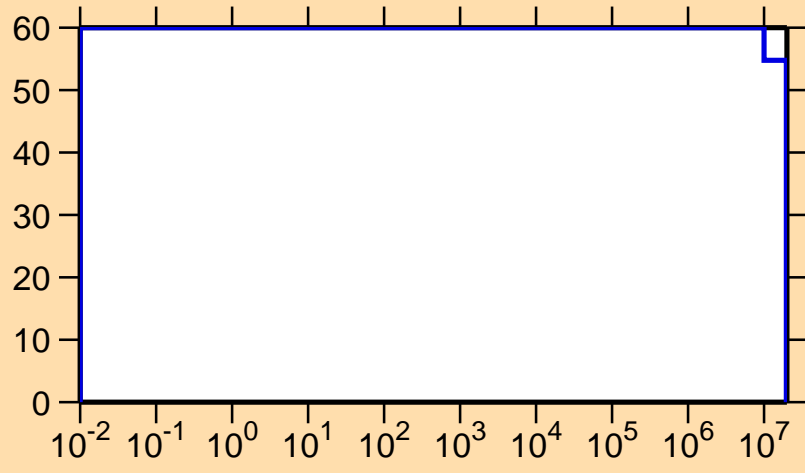
\Delta\sigma/\sigma vs. E for ^{252}\text{Md}(n,p)
