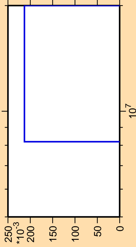
\Delta\sigma/\sigma vs. E for ^{252}\text{Md}(\text{mt117})
