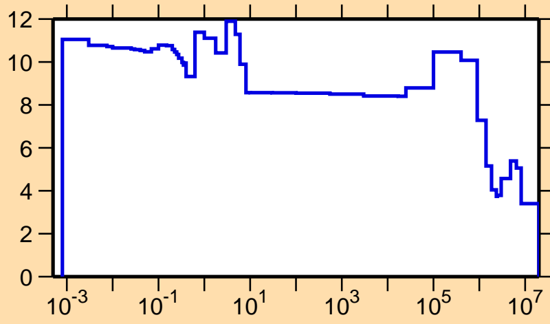
\sigma vs. E for ^{252}\text{Md}(n,\text{el.})
