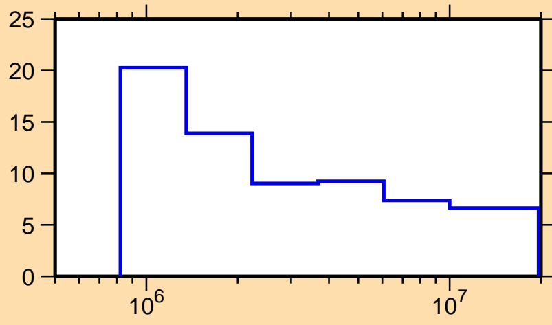
\Delta\sigma/\sigma vs. E for ^{253}\text{Md}(n,n\text{onel.})
