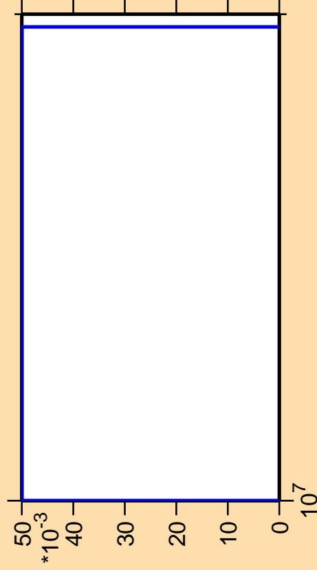
\Delta\sigma/\sigma vs. E for ^{253}\text{Md} (mt 45)
