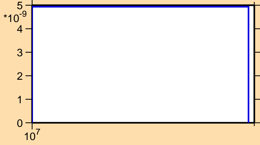
\sigma vs. E for ^{253}\text{Md}(n,2np)
