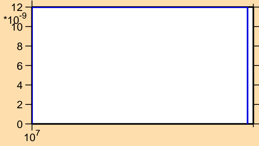
\sigma vs. E for ^{253}\text{Md}(n,\text{nd})
