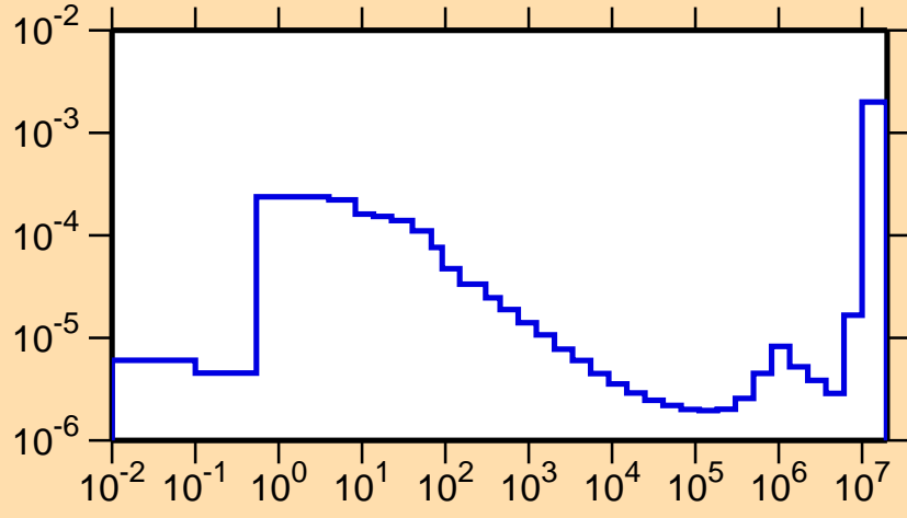
\sigma vs. E for ^{253}\text{Md}(n,\alpha)
