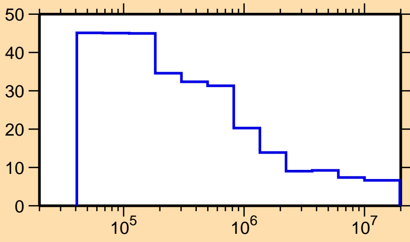
\Delta\sigma/\sigma vs. E for ^{253}\text{Md}(n,\text{nonel.})
