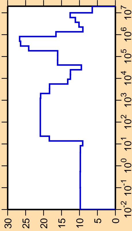
\Delta\sigma/\sigma vs. E for ^{253}\text{Md}(n,\text{el.})
