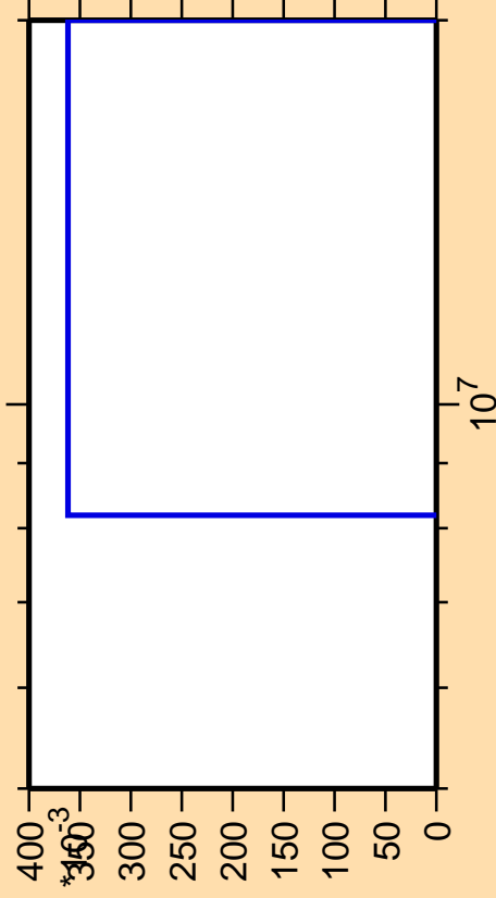
\Delta\sigma/\sigma vs. E for ^{253}\text{Md}(n,3n\alpha)
