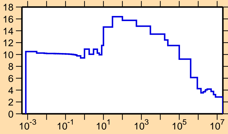
\sigma vs. E for ^{253}\text{Md}(n,\text{el.})
