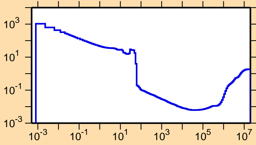
\sigma vs. E for ^{254}\text{Md}(n,f)
