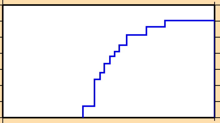
\sigma vs. E for ^{254}\text{Md}(n,3n)
