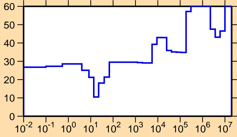
\Delta\sigma/\sigma vs. E for ^{254}\text{Md}(n,\gamma)
