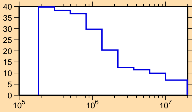
\Delta\sigma/\sigma vs. E for ^{254}\text{Md}(n,\text{nonel.})
