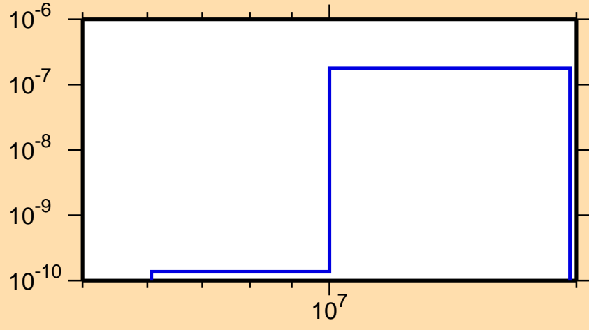
\sigma vs. E for ^{254}\text{Md}(n,2n\alpha)
