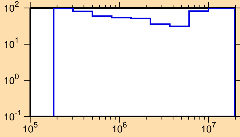
\Delta\sigma/\sigma vs. E for ^{254}\text{Md}(n,n\text{cont.})
