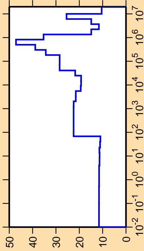
\Delta\sigma/\sigma vs. E for ^{254}\text{Md}(n,\text{el.})
