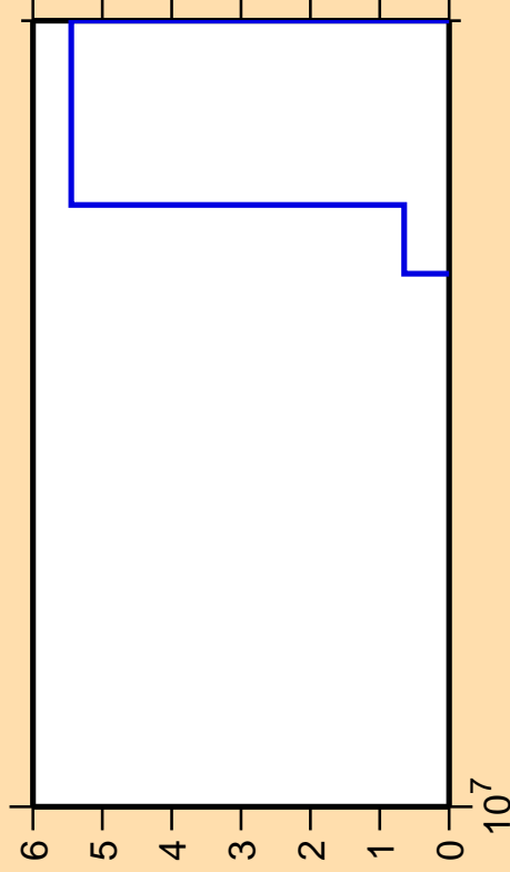
\Delta\sigma/\sigma vs. E for ^{254}\text{Md} (mt 45)
