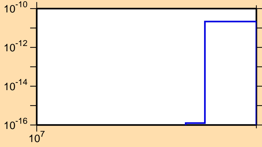
\sigma vs. E for ^{254}\text{Md} (mt 11)
