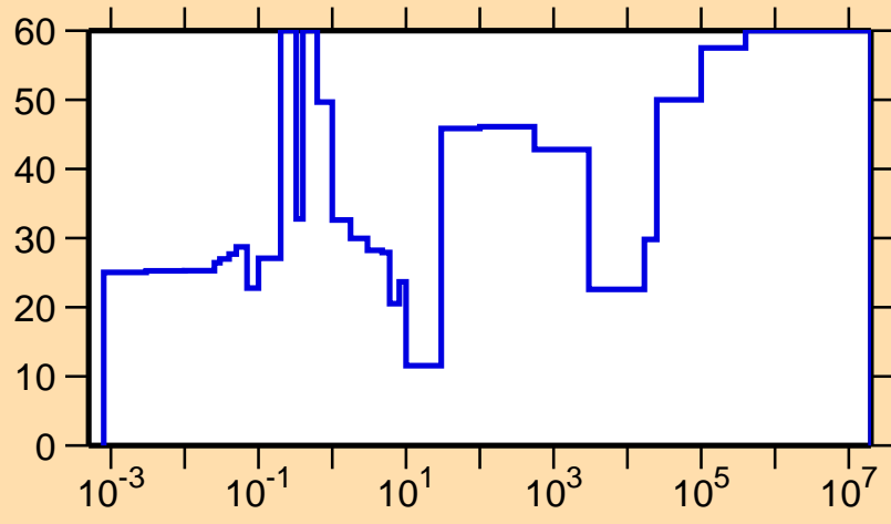
\Delta\sigma/\sigma vs. E for ^{254}\text{Md}(n,\gamma)
