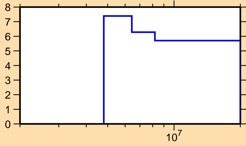
\Delta\sigma/\sigma vs. E for ^{254}\text{Md}(n,\text{nonel.})
