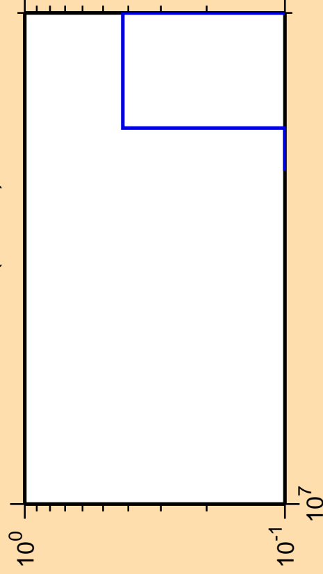
\Delta\sigma/\sigma vs. E for ^{255}\text{Md} (mt 11)
