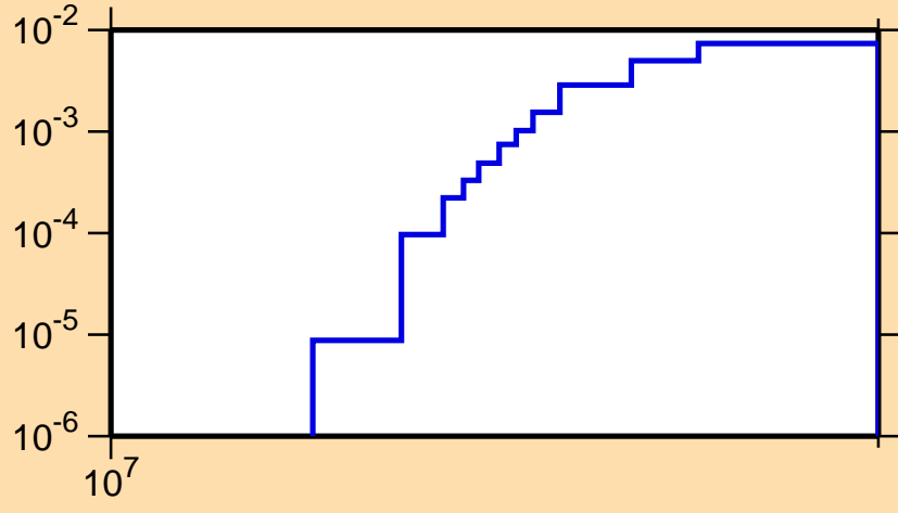
\sigma vs. E for ^{255}\text{Md}(n,3n)
