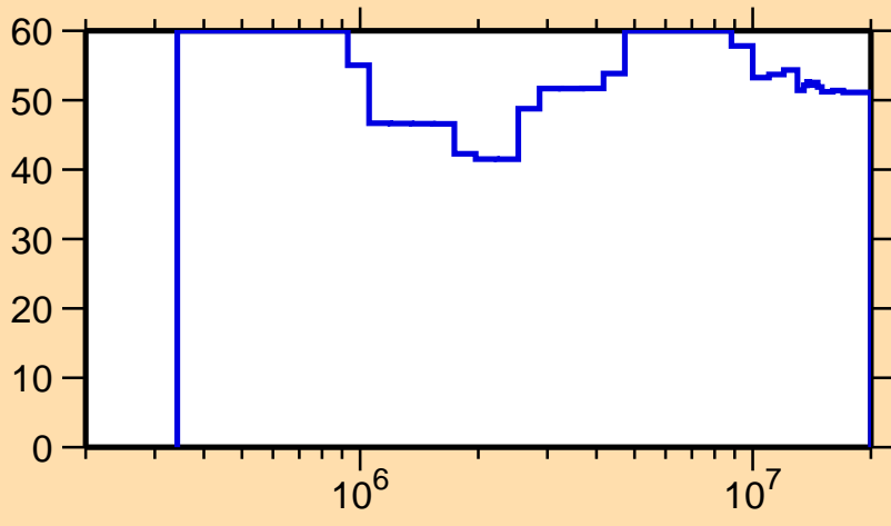
\Delta\sigma/\sigma vs. E for ^{255}\text{Md}(n,ncont.)
