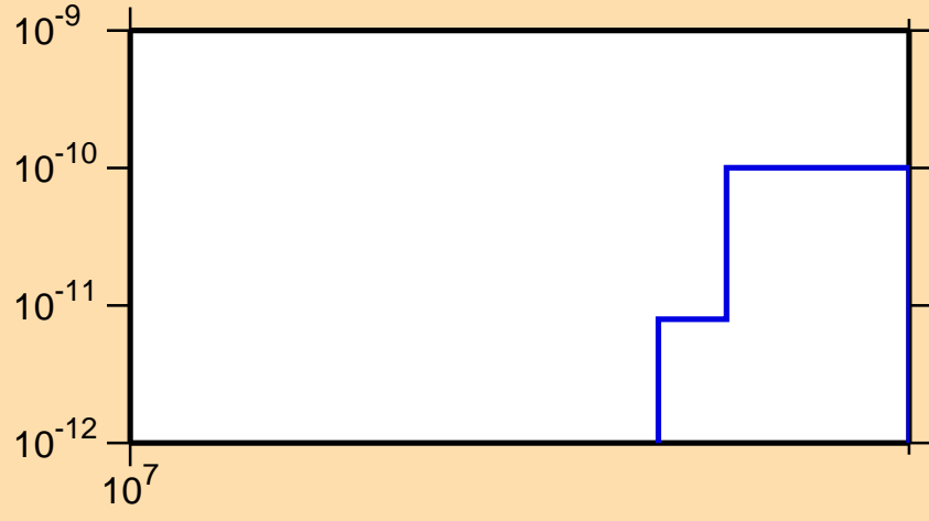
\sigma vs. E for ^{255}\text{Md}(\text{mt117})
