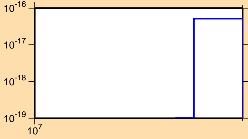
\sigma vs. E for ^{255}\text{Md} (mt 34)
