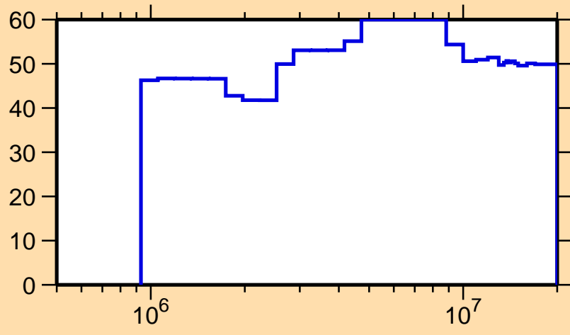
\Delta\sigma/\sigma vs. E for ^{255}\text{Md}(n,\text{inel.})
