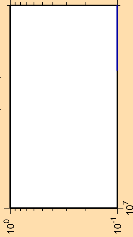
\Delta\sigma/\sigma vs. E for ^{255}\text{Md} (mt 34)
