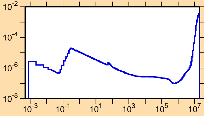
\sigma vs. E for ^{255}\text{Md}(n,\alpha)
