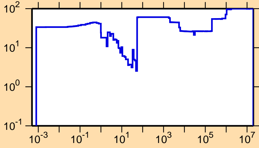
\Delta\sigma/\sigma vs. E for ^{255}\text{Md}(n,\gamma)
