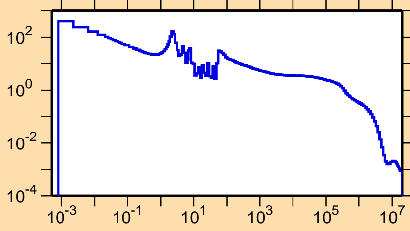
\sigma vs. E for ^{255}\text{Md}(n,\gamma)
