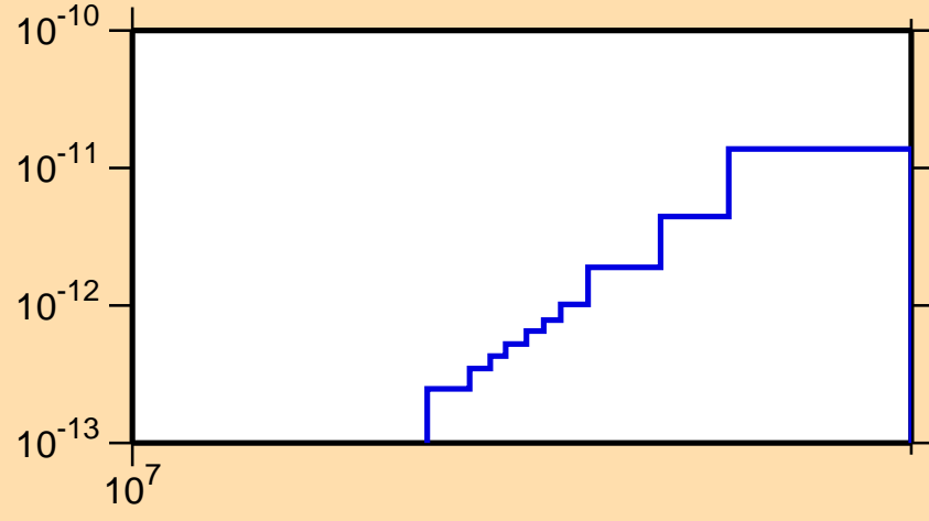
\sigma vs. E for ^{255}\text{Md}(n,p\alpha)
